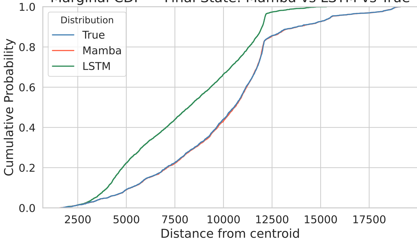
Marginal CDF — Final State: Mamba vs LSTM vs True
