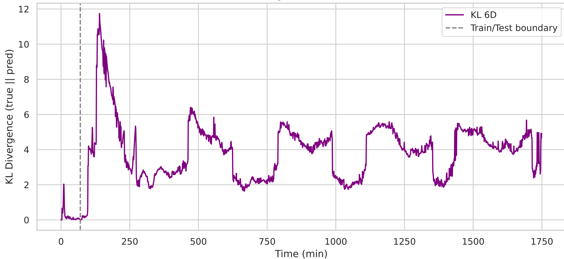
Full 6D KL Divergence: lstm — KL=4.9053
