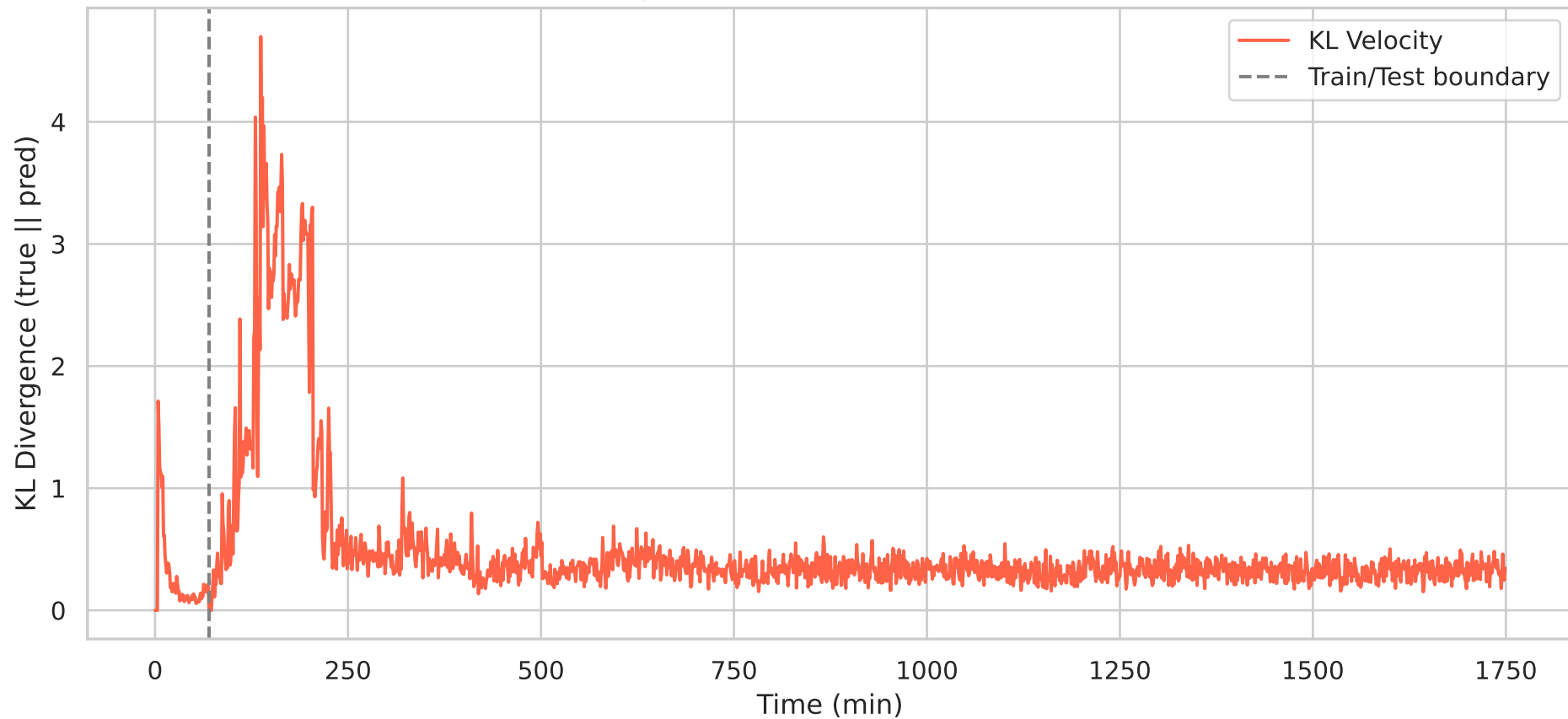
Final Velocity KL Divergence: Istm — Vel KL=0.3443
