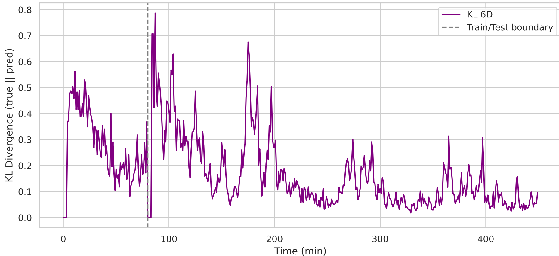
Full 6D KL Divergence: lstm — KL=0.0972
