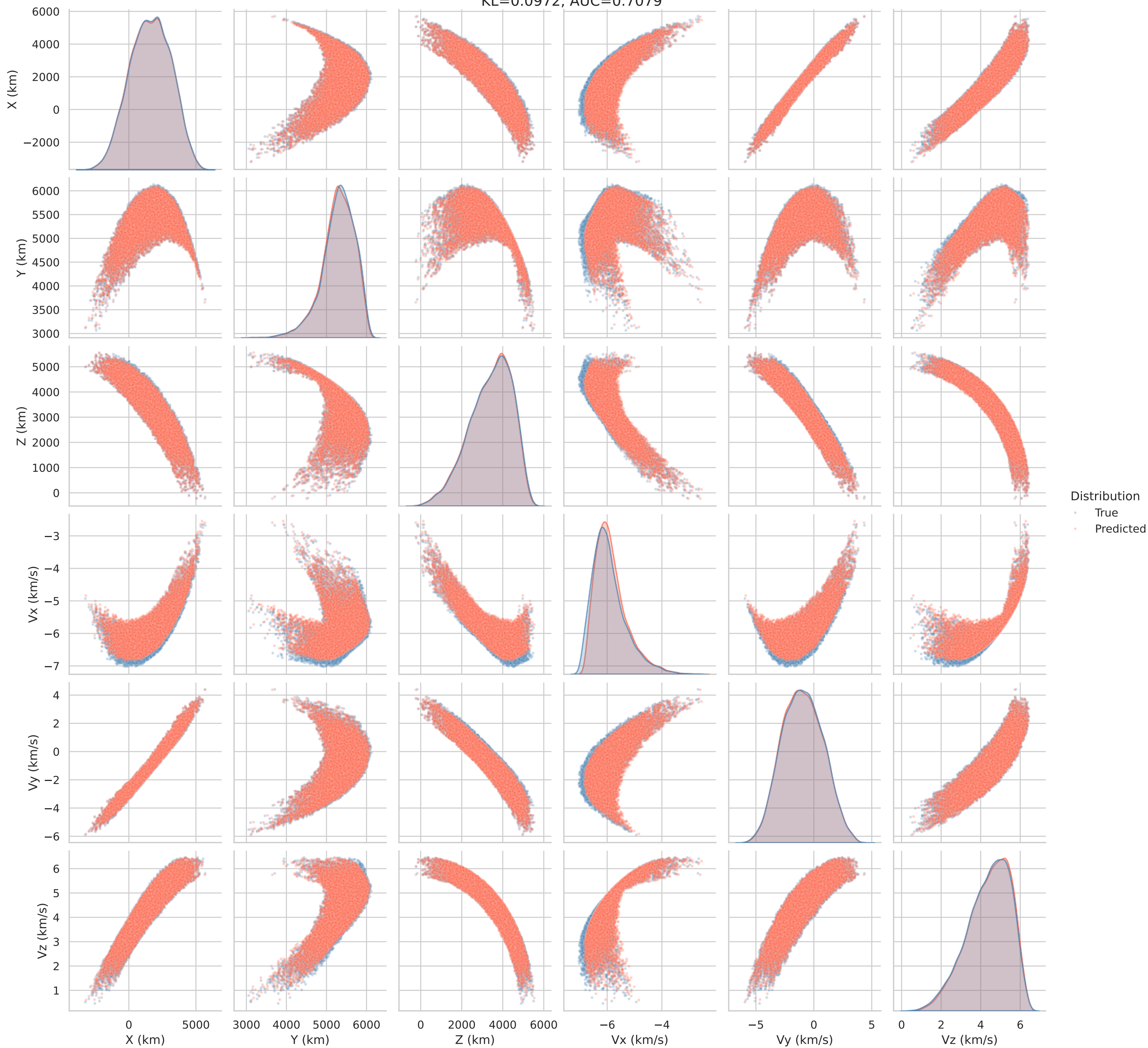
Istm Final State Pairplot — True vs Predicted KL=0.0972, AUC=0.7079
