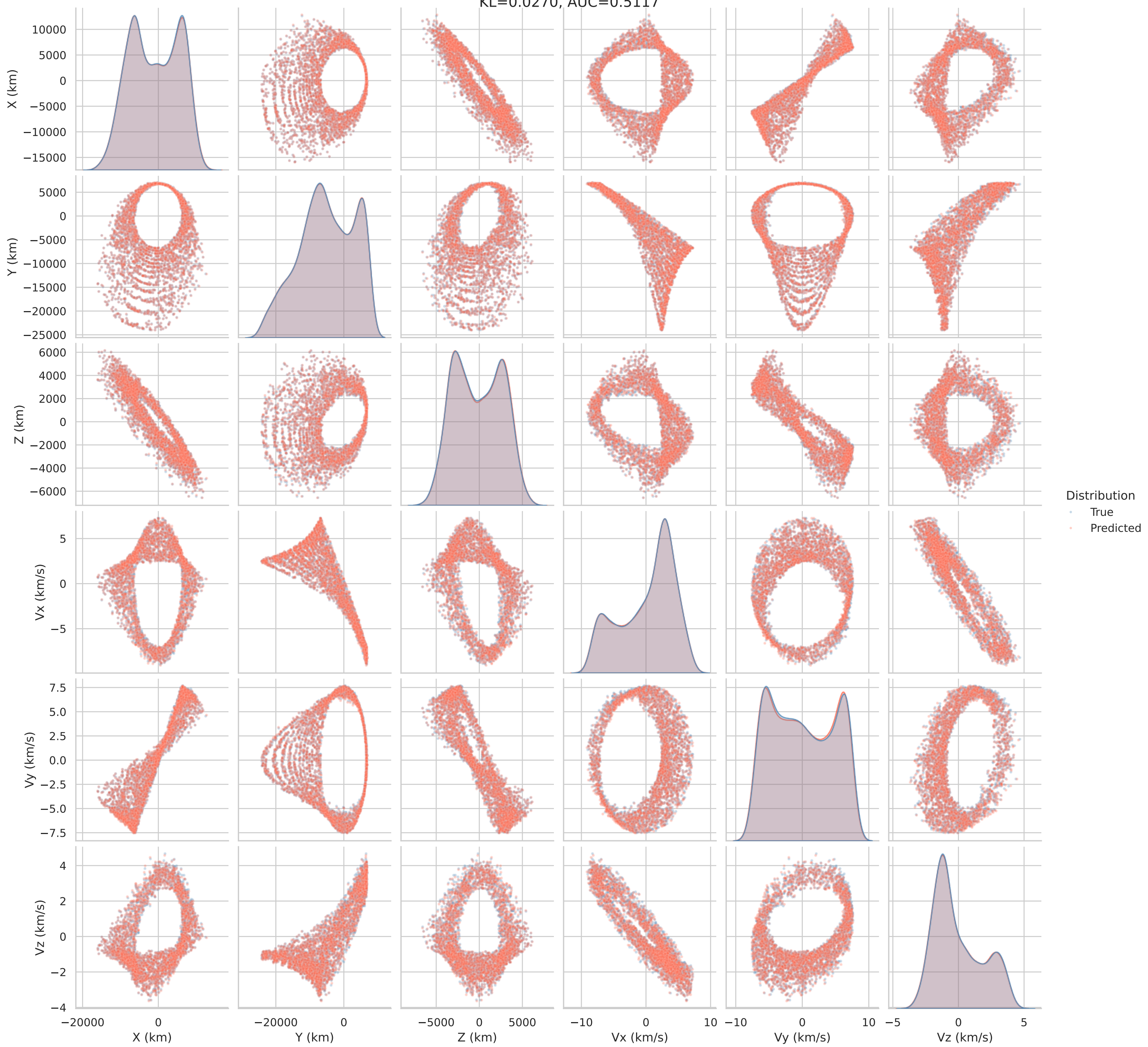
mamba Final State Pairplot — True vs Predicted KL=0.0270, AUC=0.5117
