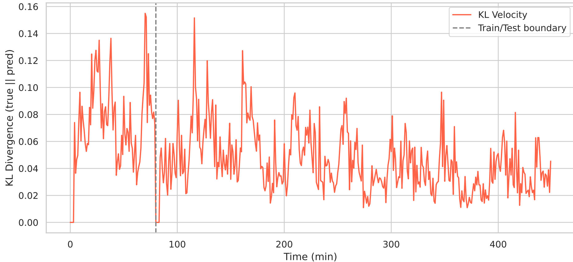
Final Velocity KL Divergence: mamba — Vel KL=0.0454
