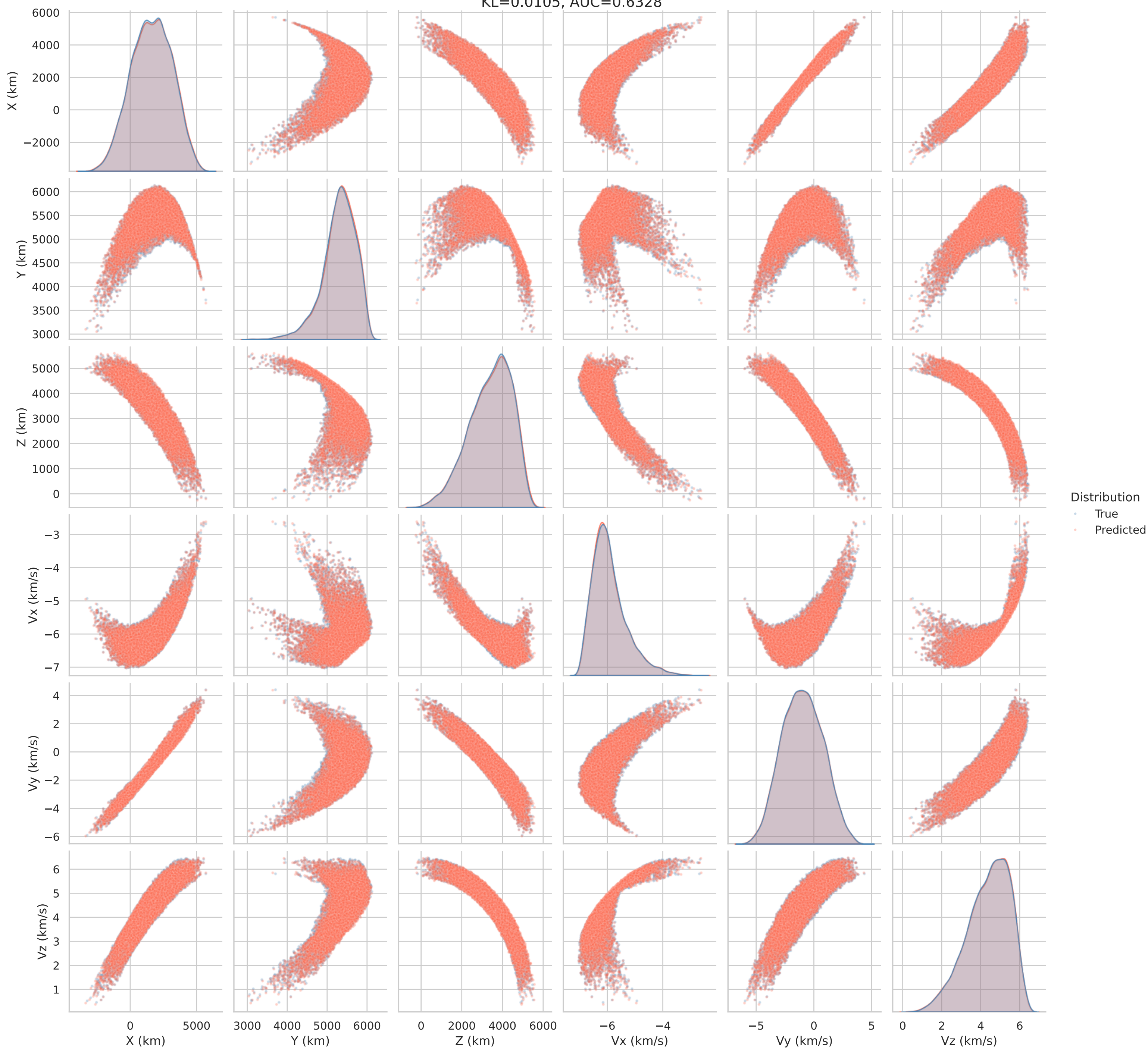
mamba Final State Pairplot — True vs Predicted KL=0.0105, AUC=0.6328
