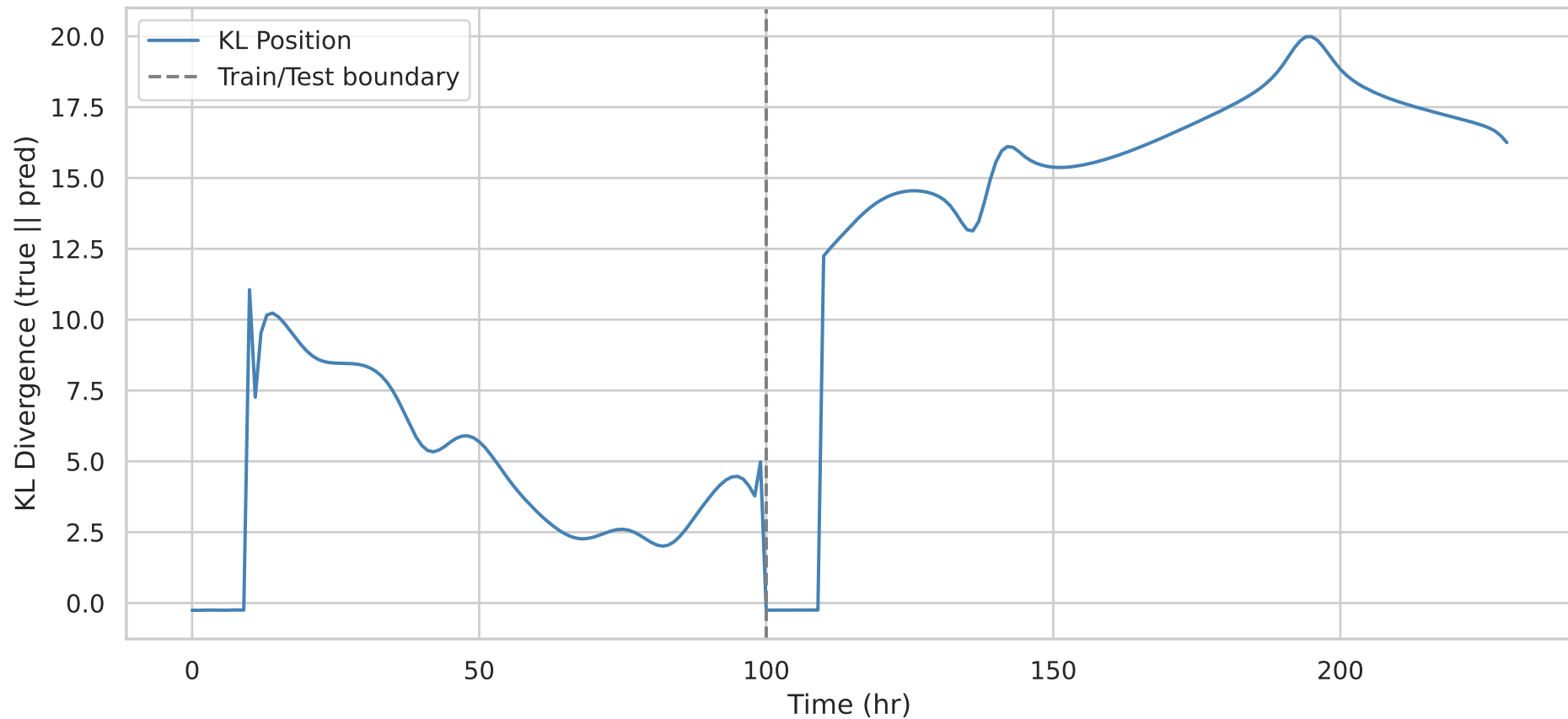
Final Position KL Divergence: lstm — Pos KL=16.2508
