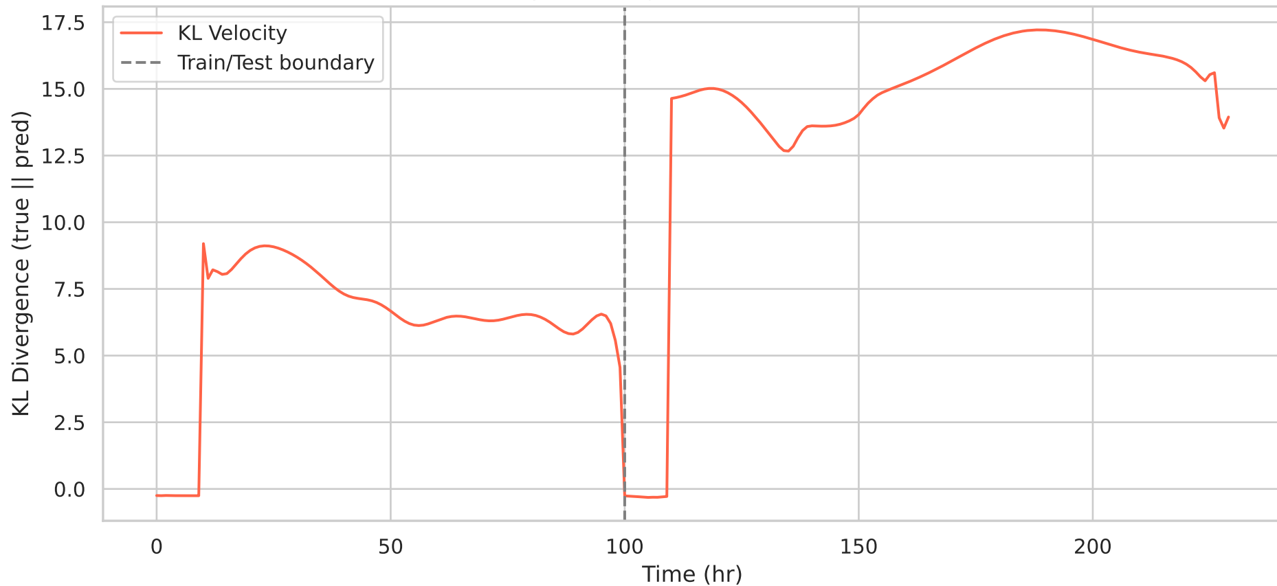
Final Velocity KL Divergence: lstm — Vel KL=13.9465
