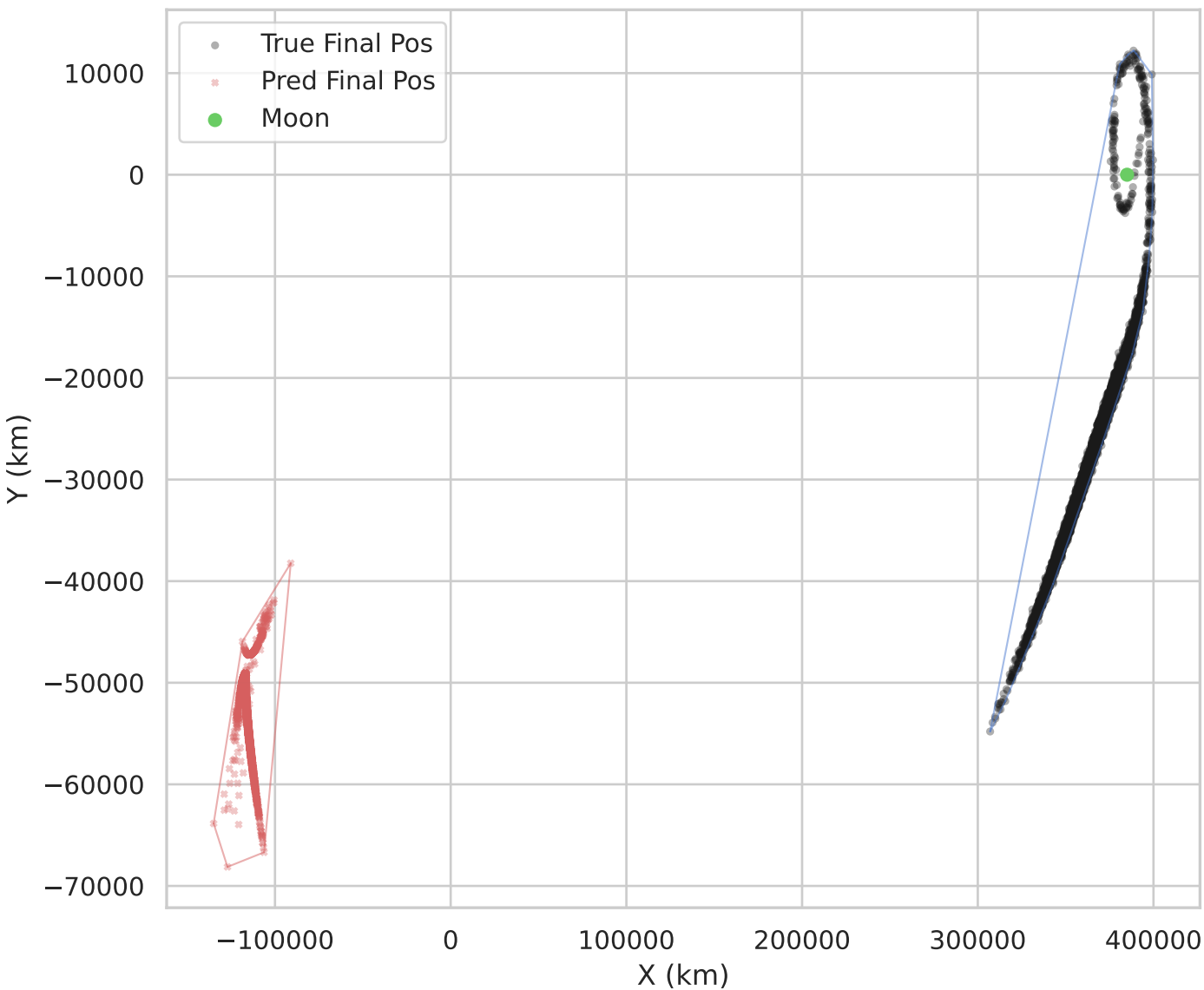
Istm Final-State Positions Convex Hull Area Ratio (Pred/True): 0.3759
