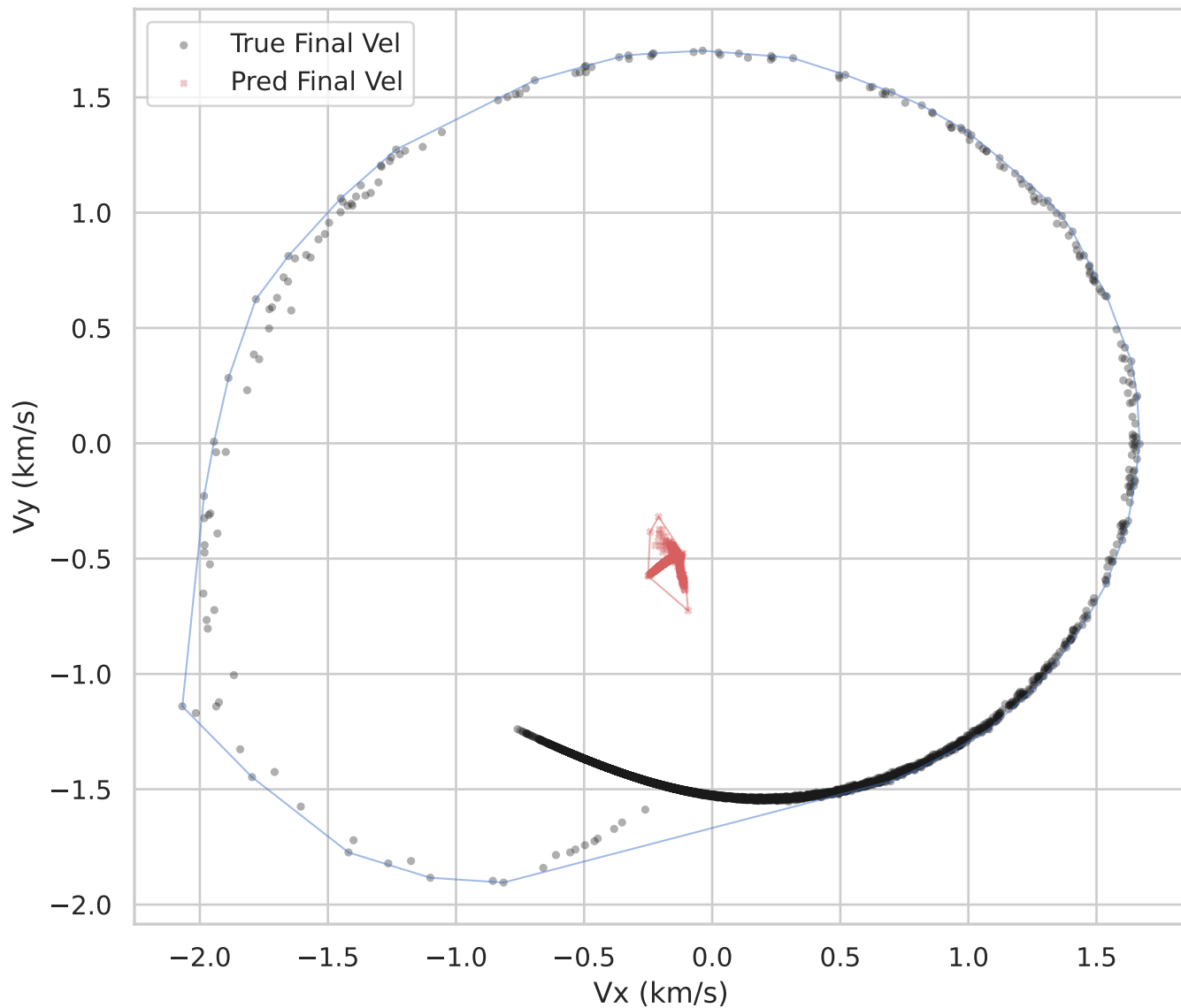
Istm Final-State Velocities Convex Hull Area Ratio (Pred/True): 0.0035
