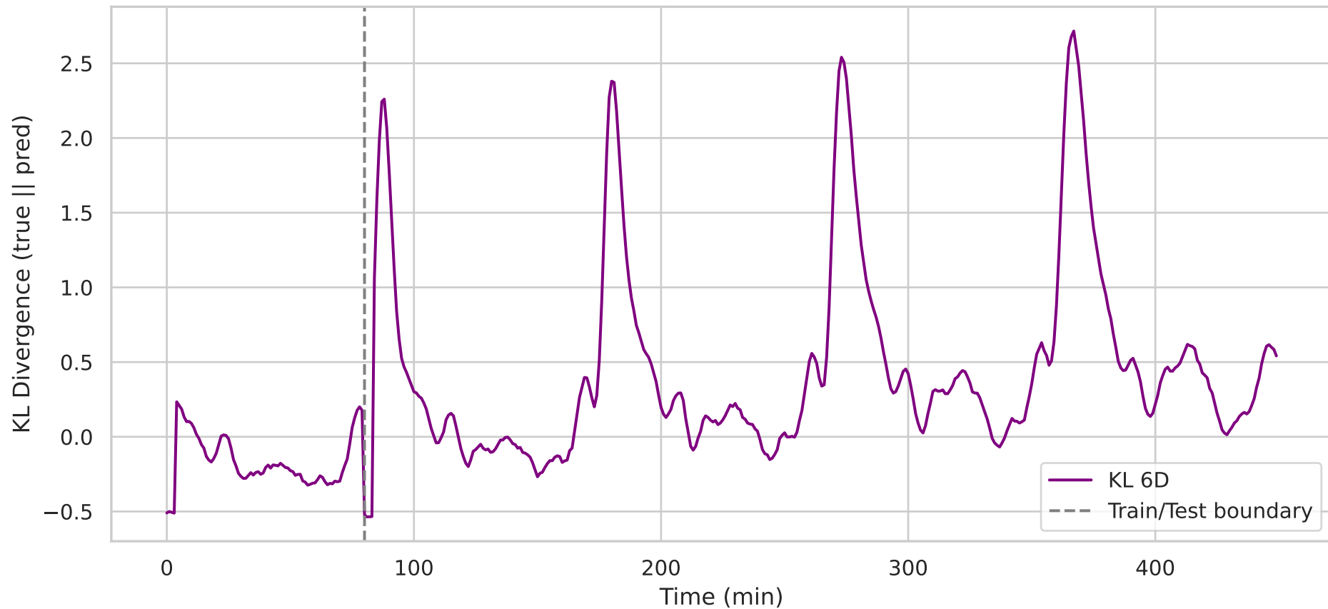
Full 6D KL Divergence: Istm — KL=0.5413
