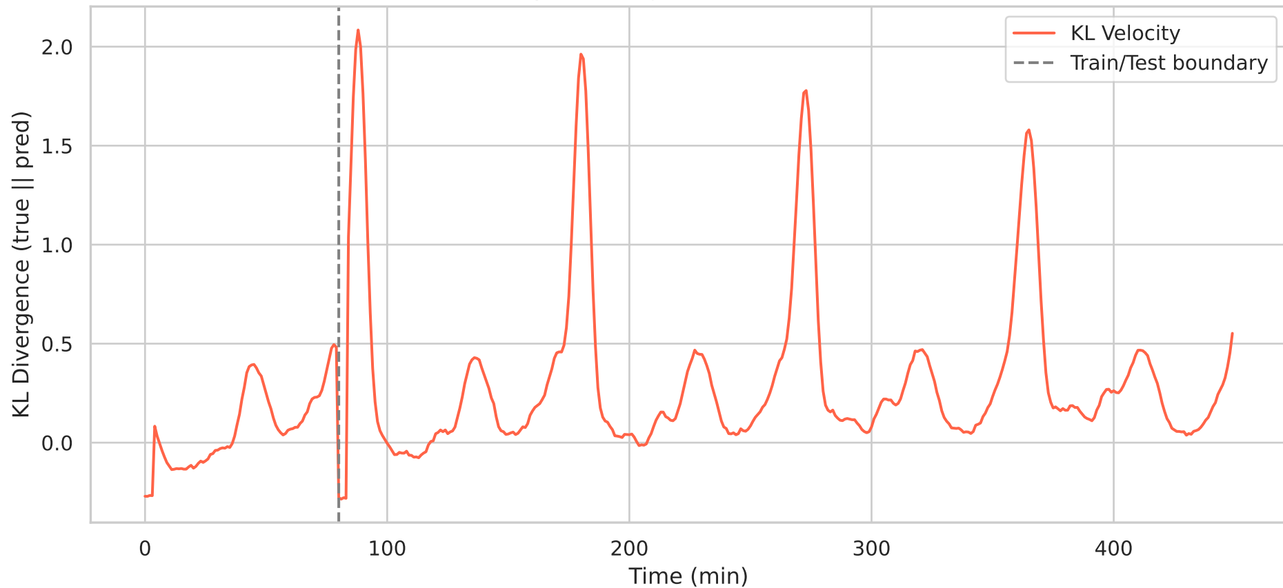
Final Velocity KL Divergence: lstm — Vel KL=0.5521
