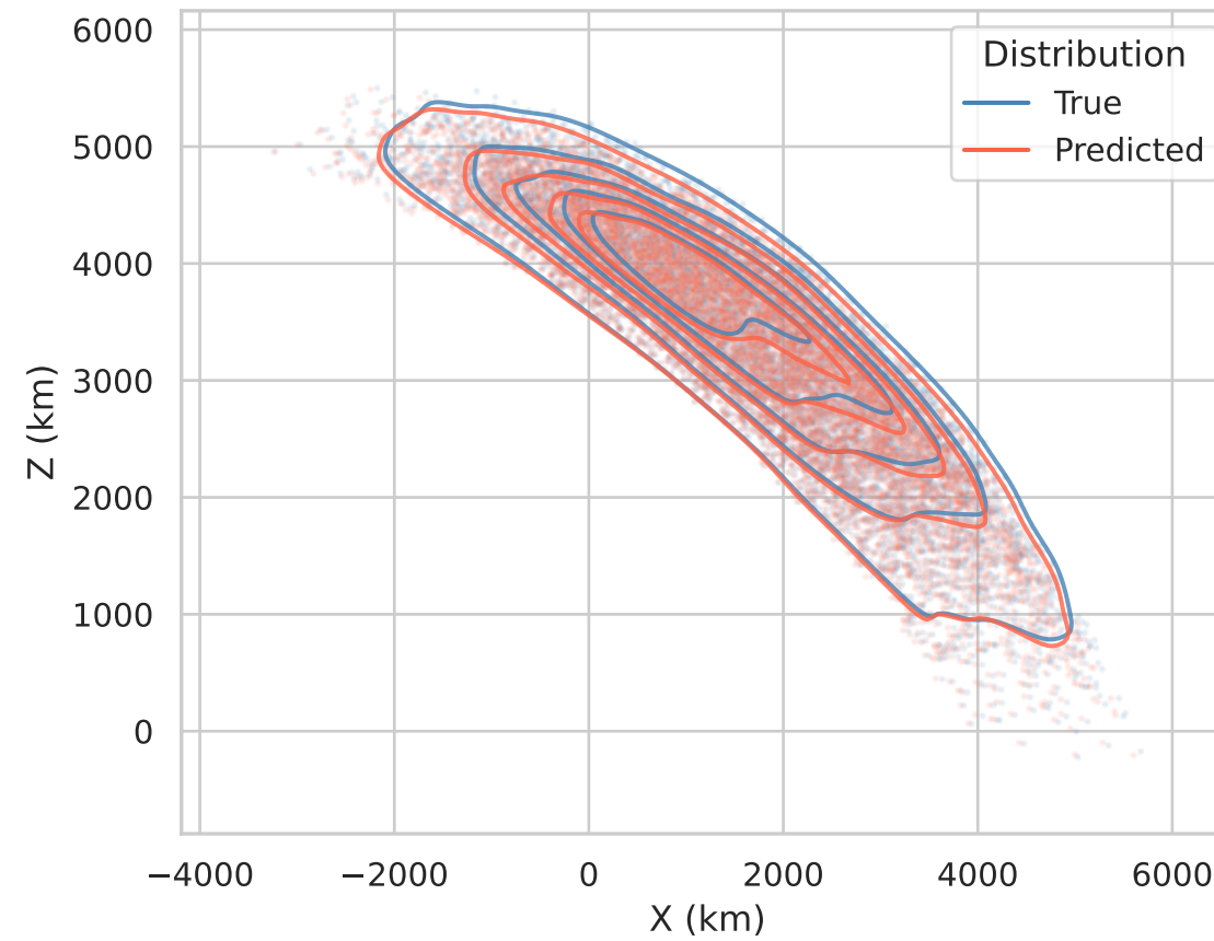
Final Reachable Set PDF: lstm KL=0.5413 — AUC=0.6405
