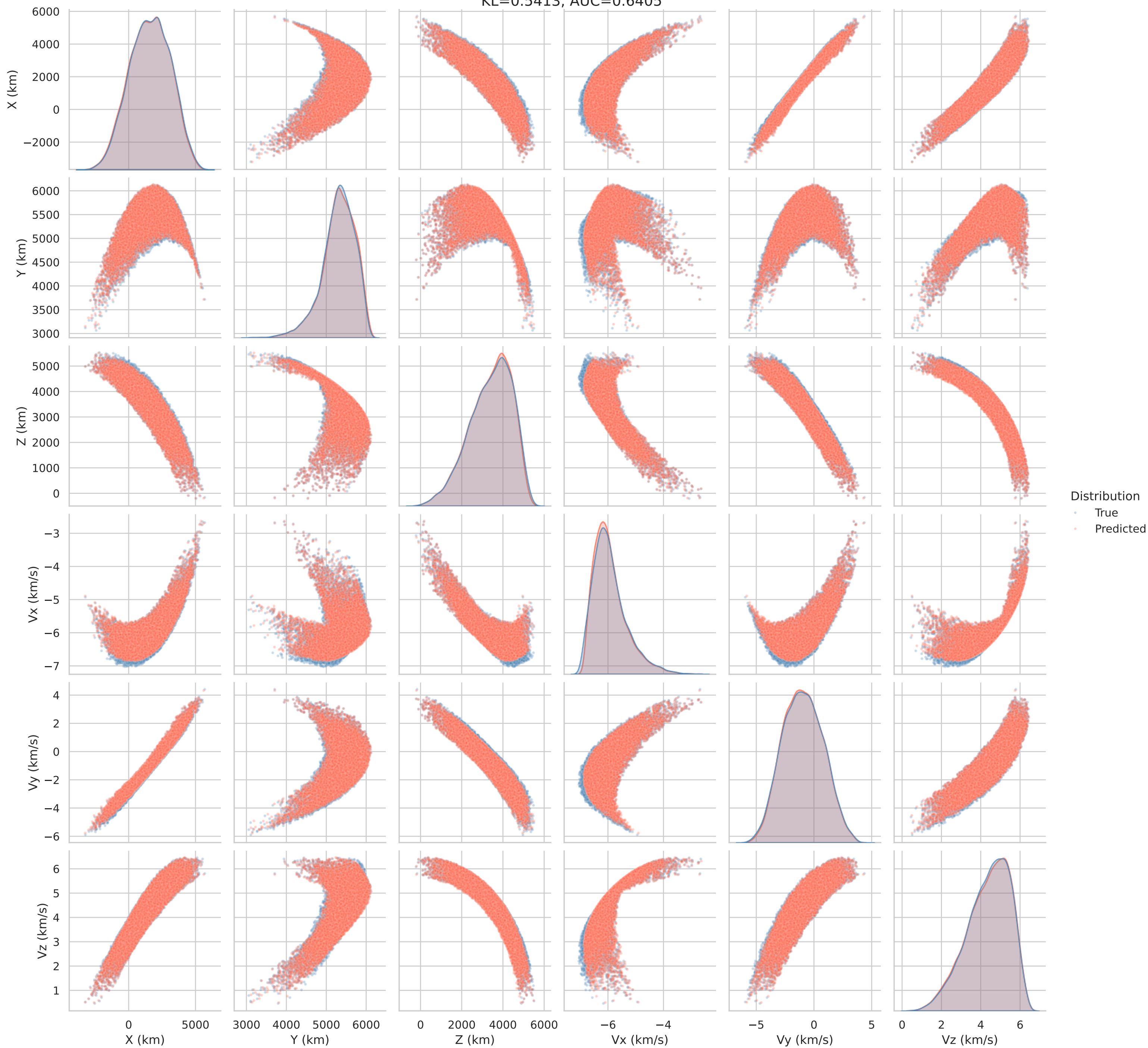
Istm Final-State Pairplot — True vs Predicted KL=0.5413, AUC=0.6405
