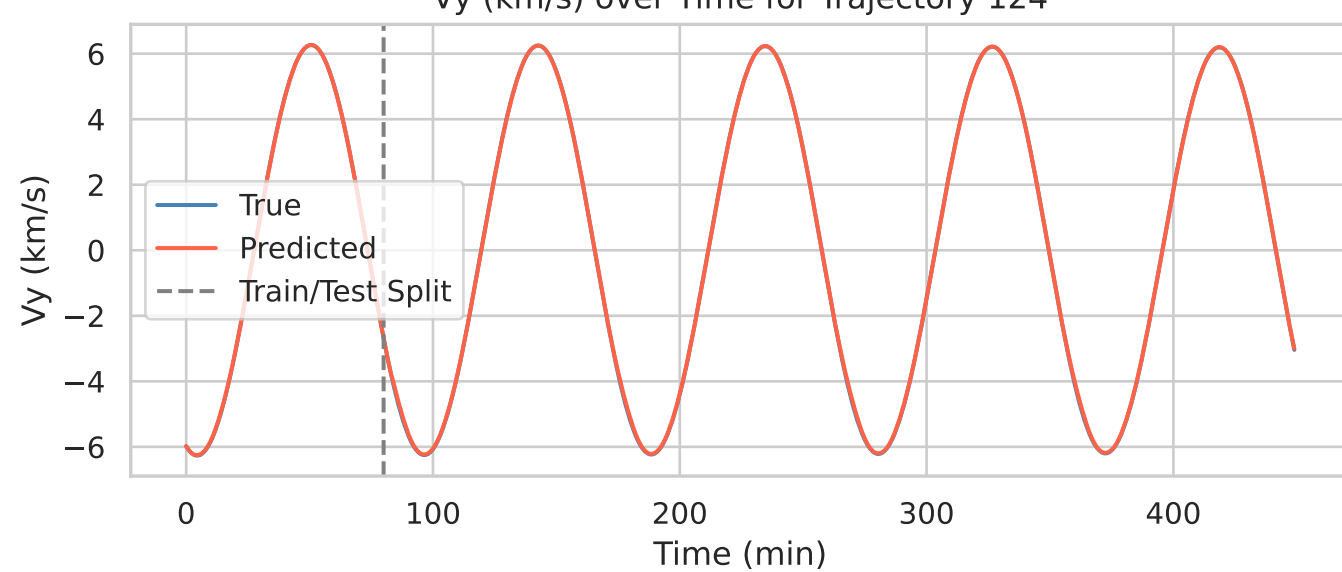
Vy (km/s) over Time for Trajectory 124
