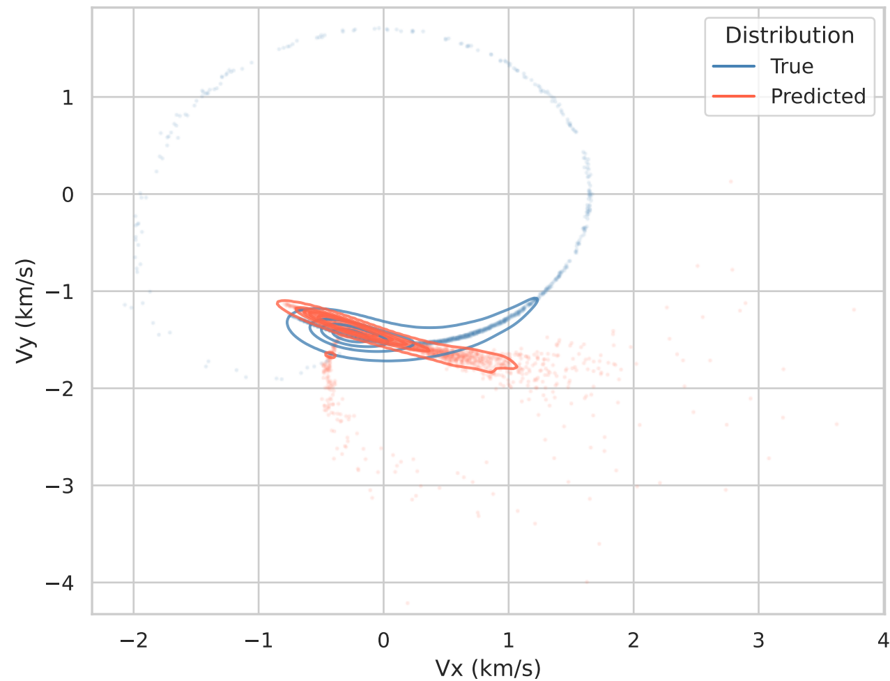
Final Reachable Set PDF: mamba KL=12.4540 — AUC=1.0000
