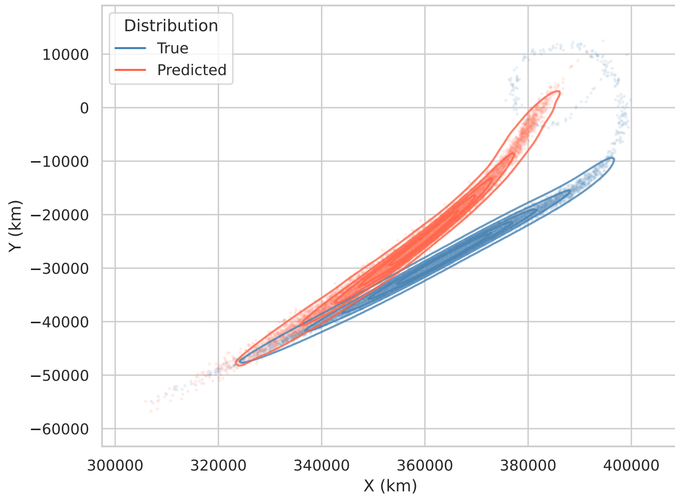
Final Reachable Set PDF: mamba KL=12.4540 — AUC=1.0000
