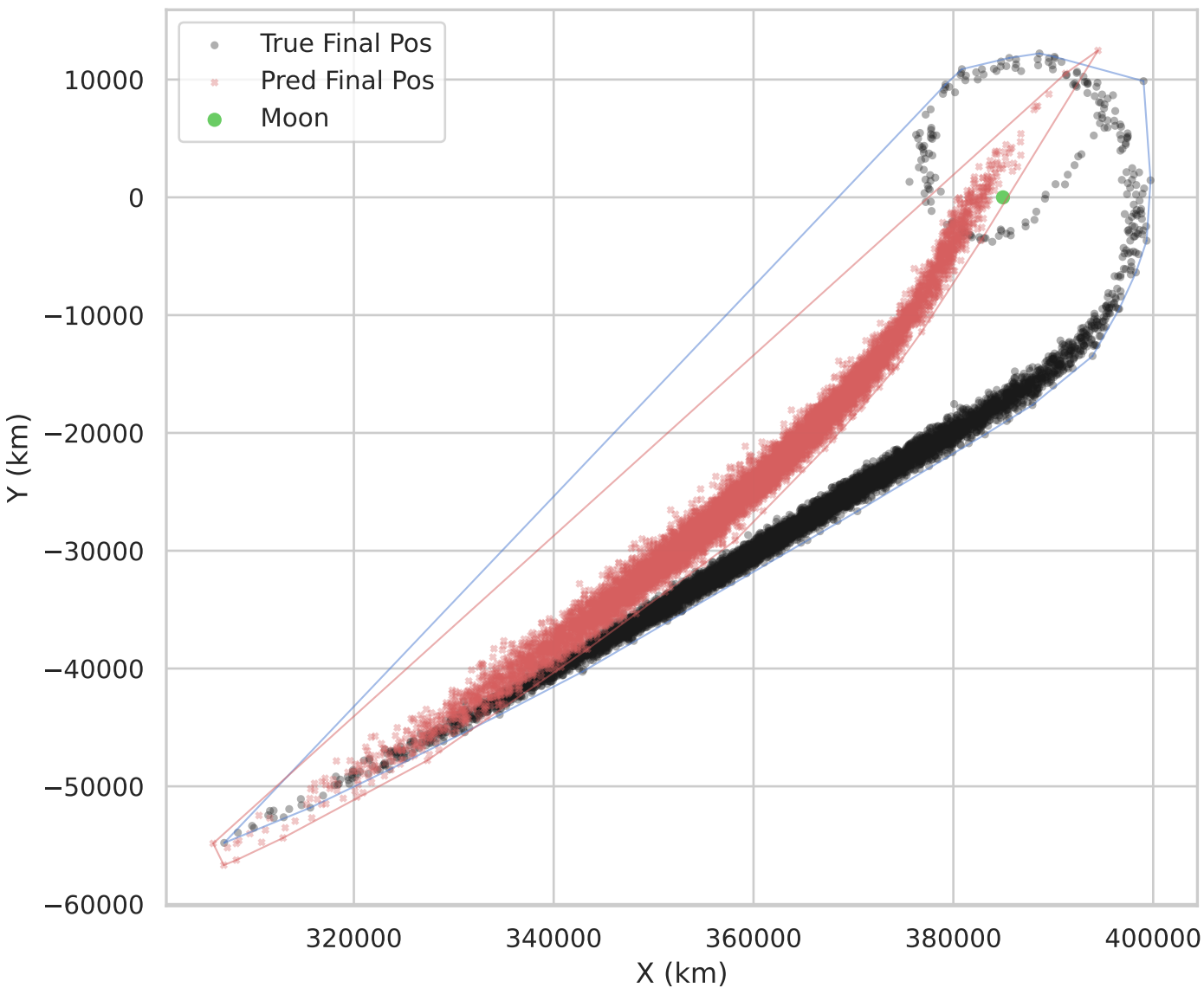
mamba Final-State Positions Convex Hull Area Ratio (Pred/True): 0.4783
