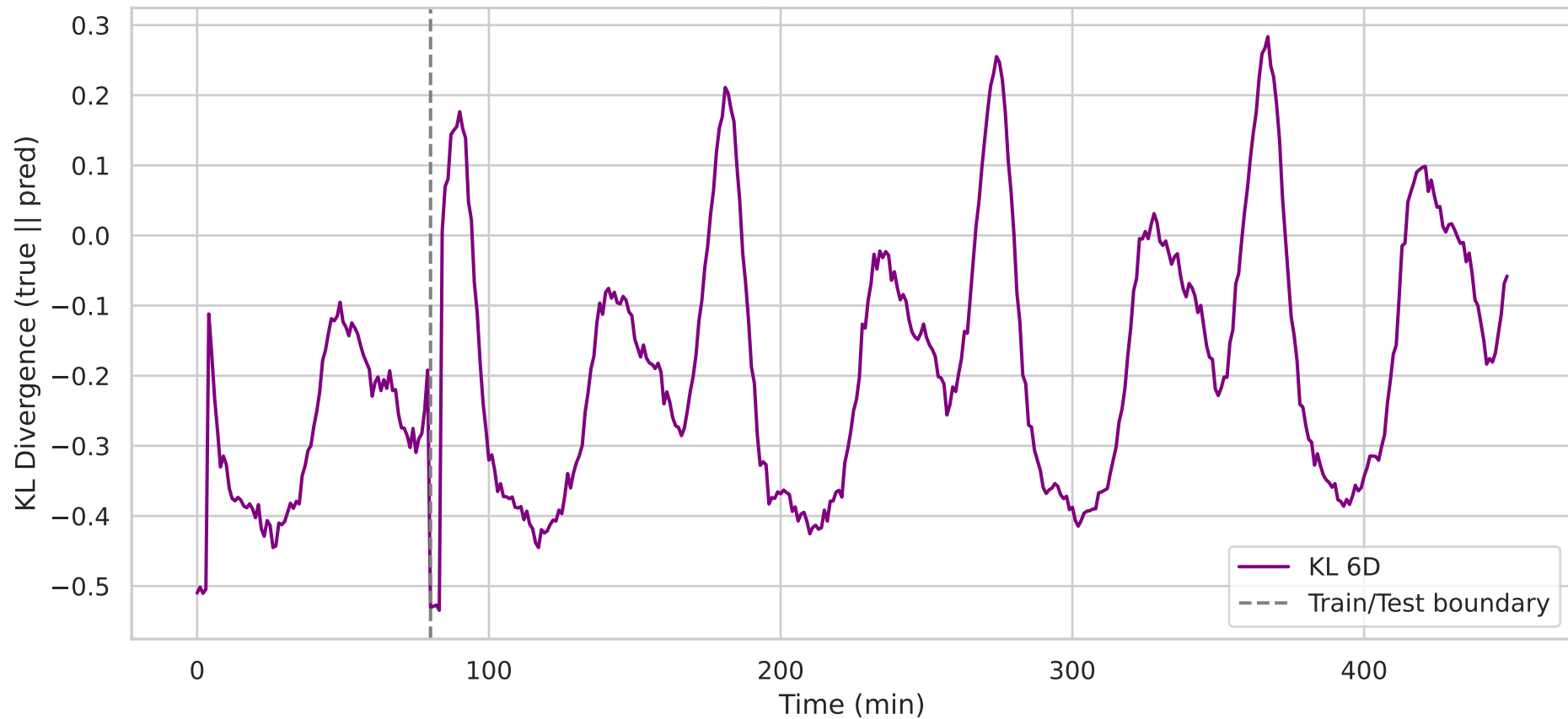
Full 6D KL Divergence: mamba — KL=-0.0579
