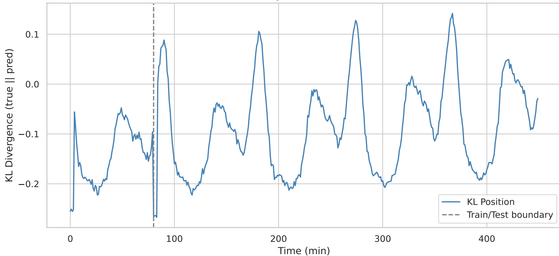
Final Position KL Divergence: mamba — Pos KL=-0.0289
