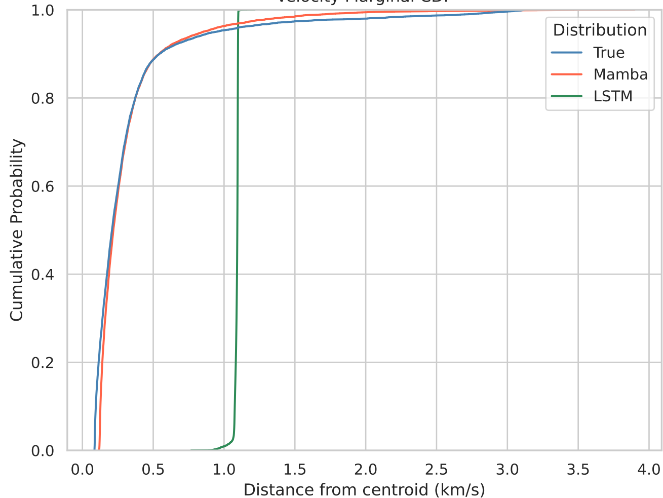
Velocity Marginal CDF
