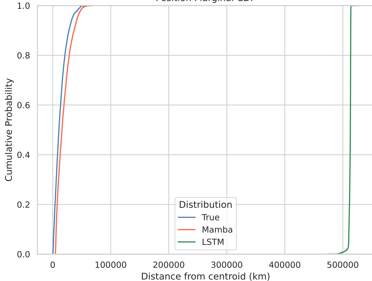
Position Marginal CDF
