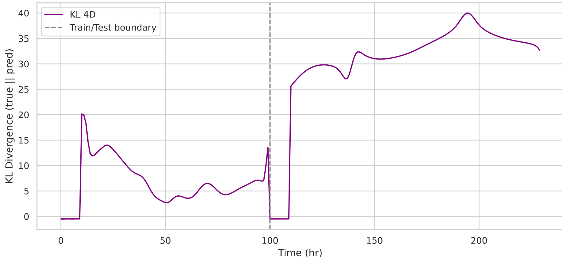
Full 4D KL Divergence: lstm — KL=32.6906
