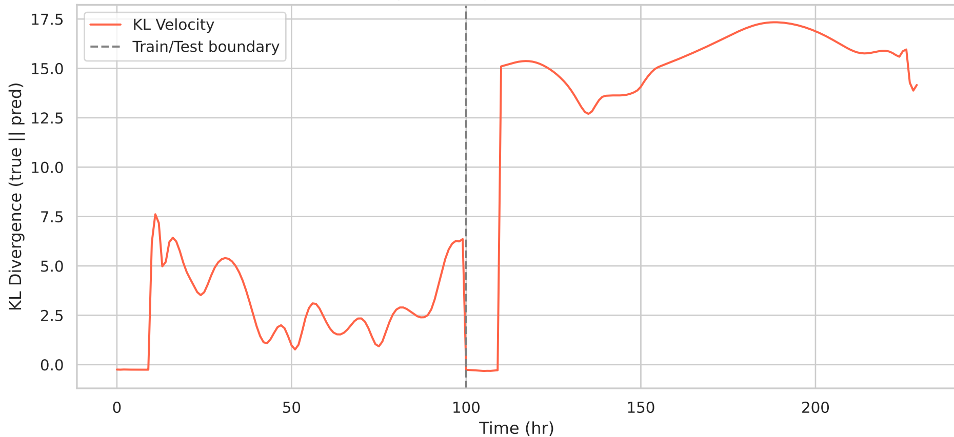
Final Velocity KL Divergence: lstm — Vel KL=14.1589
