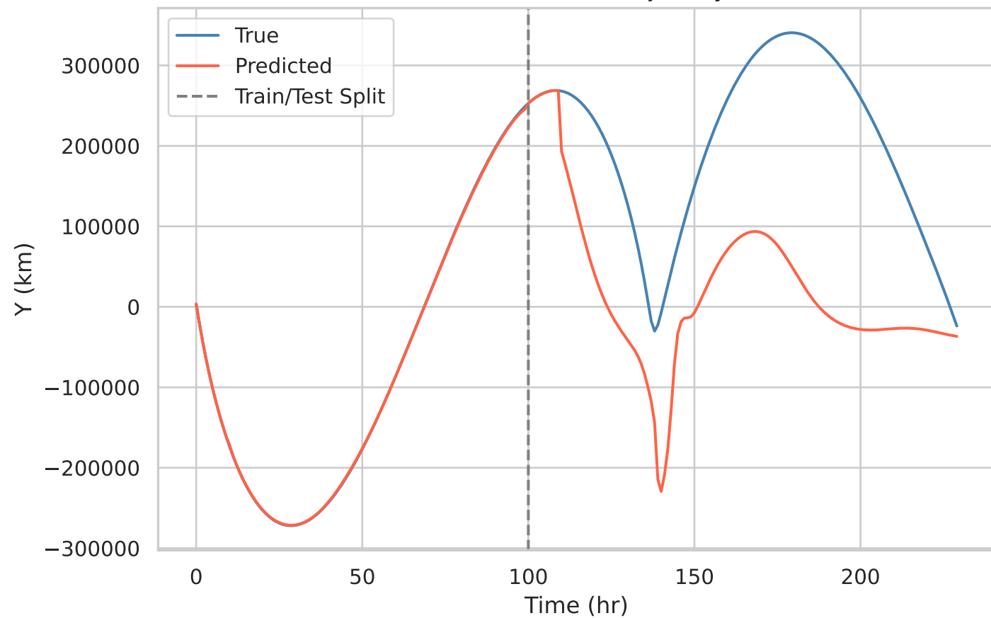
Y (km) over Time for Trajectory 124
