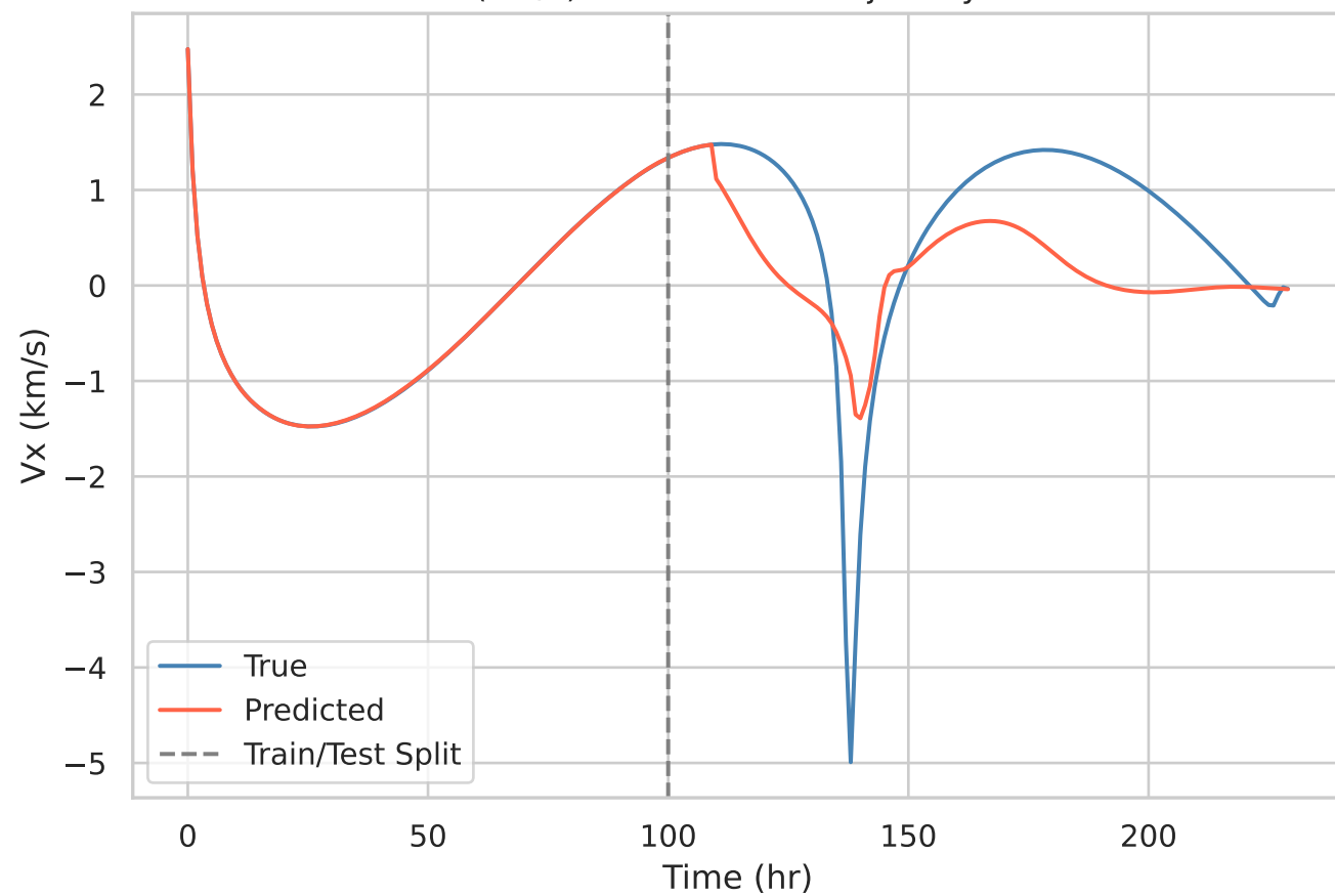
Vx (km/s) over Time for Trajectory 124
