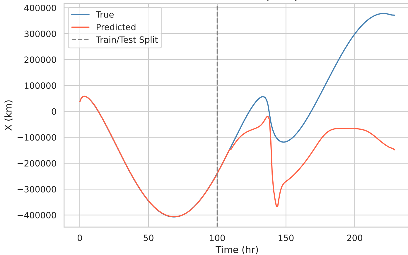
X (km) over Time for Trajectory 124
