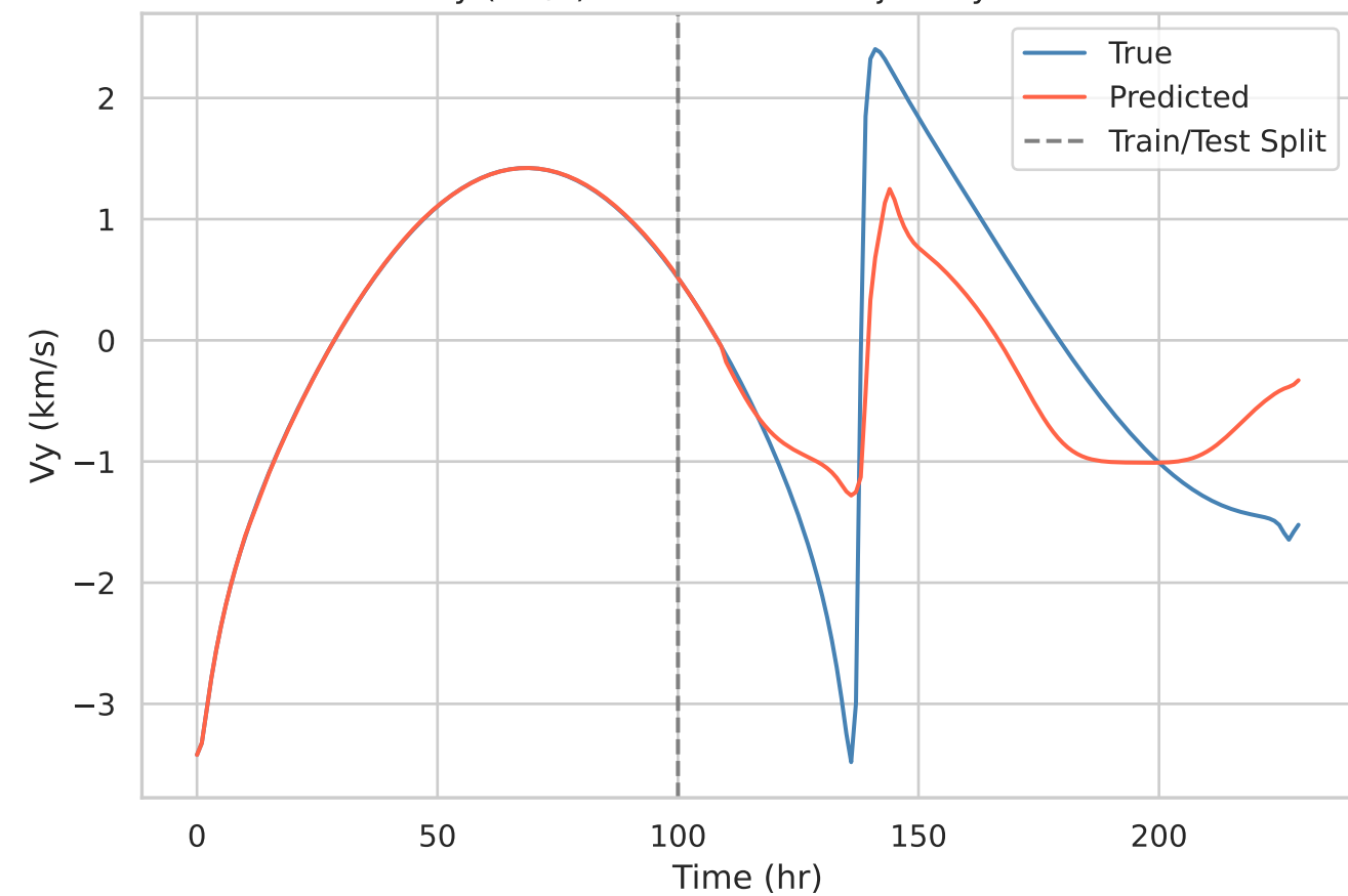
Vy (km/s) over Time for Trajectory 124
