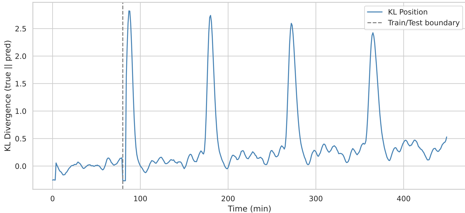
Final Position KL Divergence: lstm — Pos KL=0.5293
