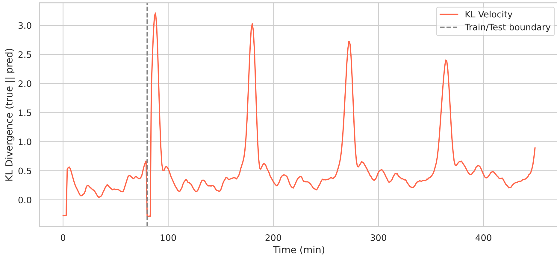
Final Velocity KL Divergence: lstm — Vel KL=0.8964
