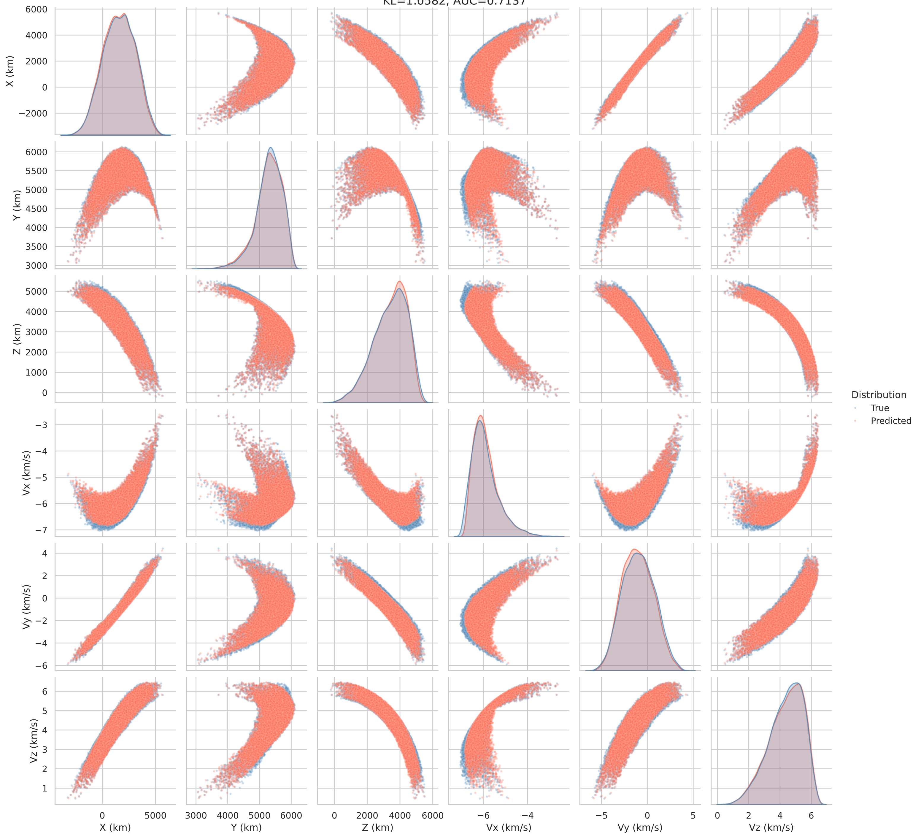
Istm Final State Pairplot — True vs Predicted KL=1.0582, AUC=0.7137
