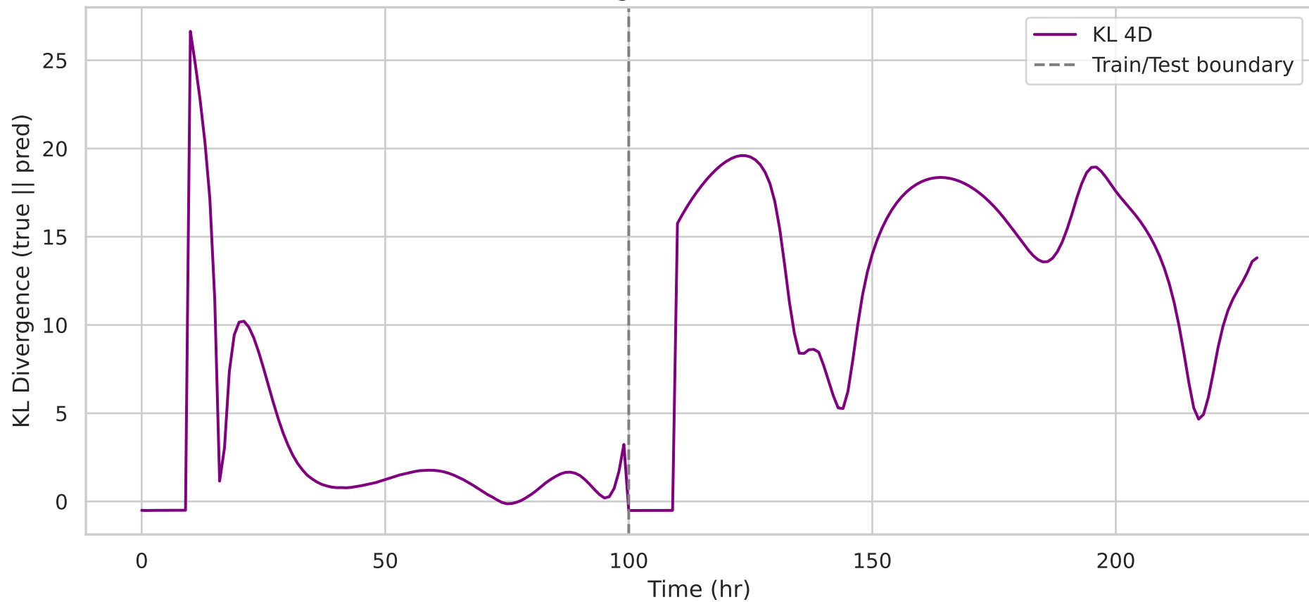
Full 4D KL Divergence: mamba — KL=13.8084
