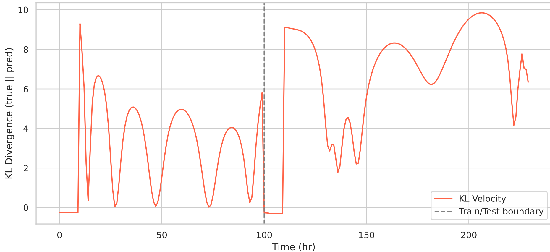
Final Velocity KL Divergence: mamba — Vel KL=6.3453
