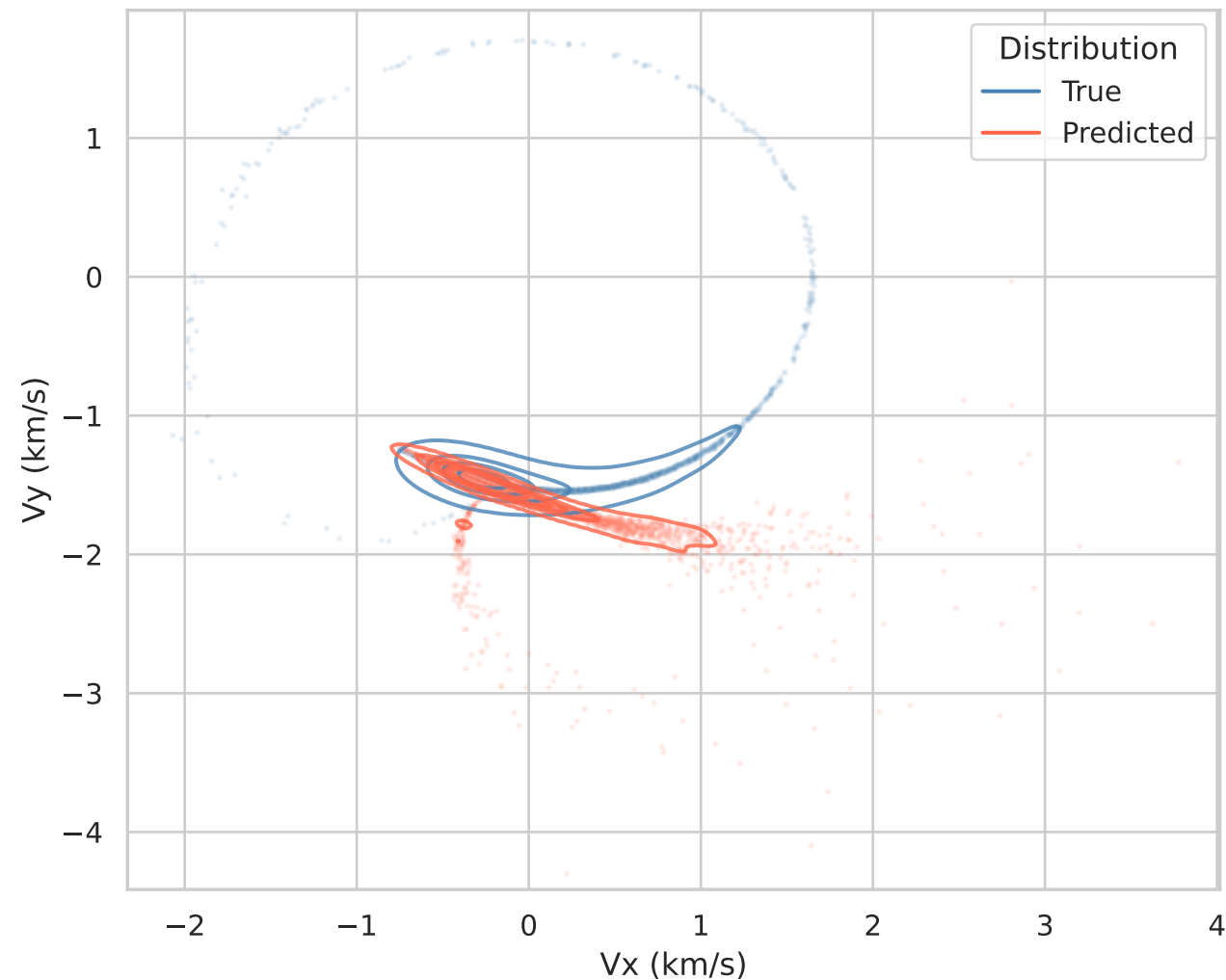
Final State PDF: mamba
