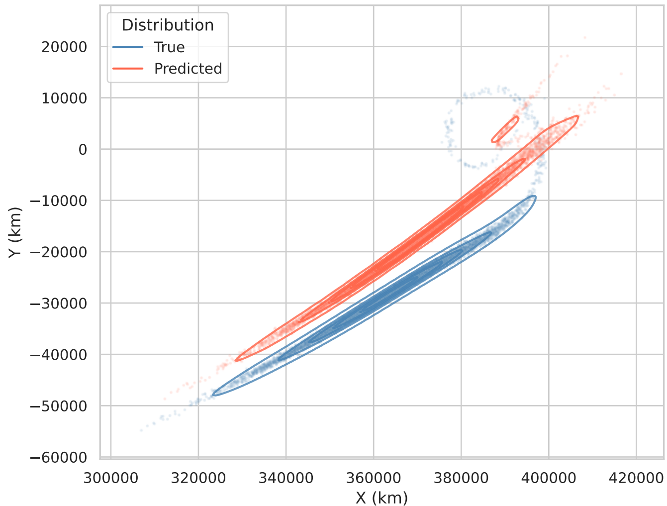
Final State PDF: mamba
