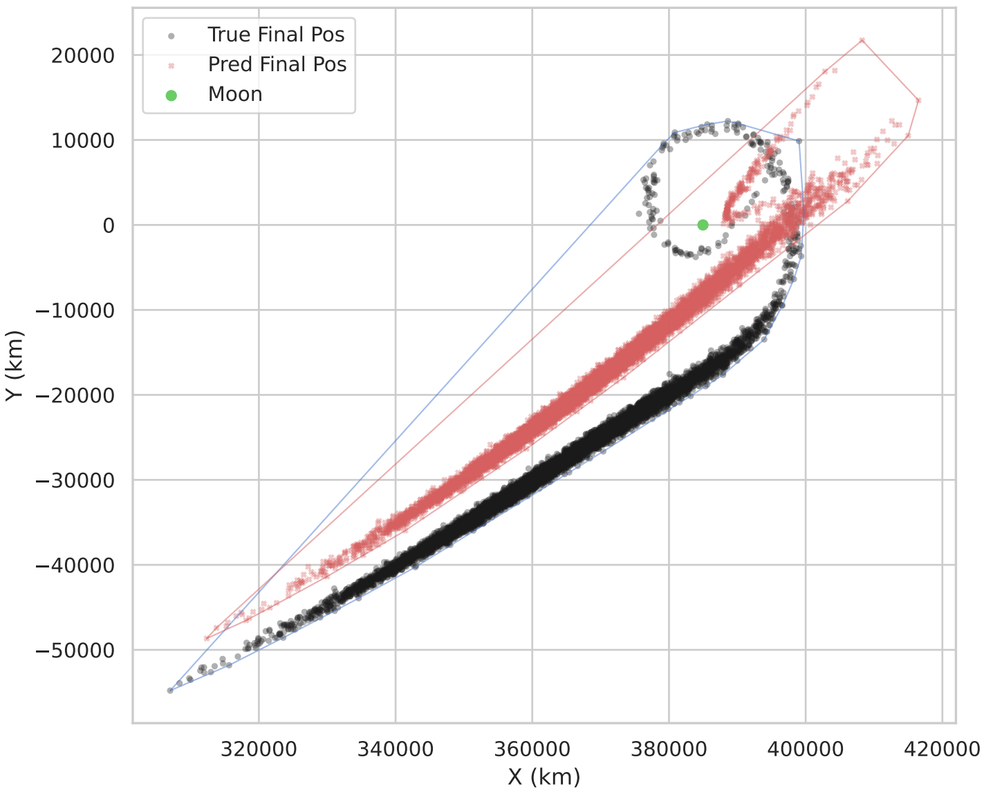
mamba Final State Positions Convex Hull Area Ratio (Pred/True): 0.6571
