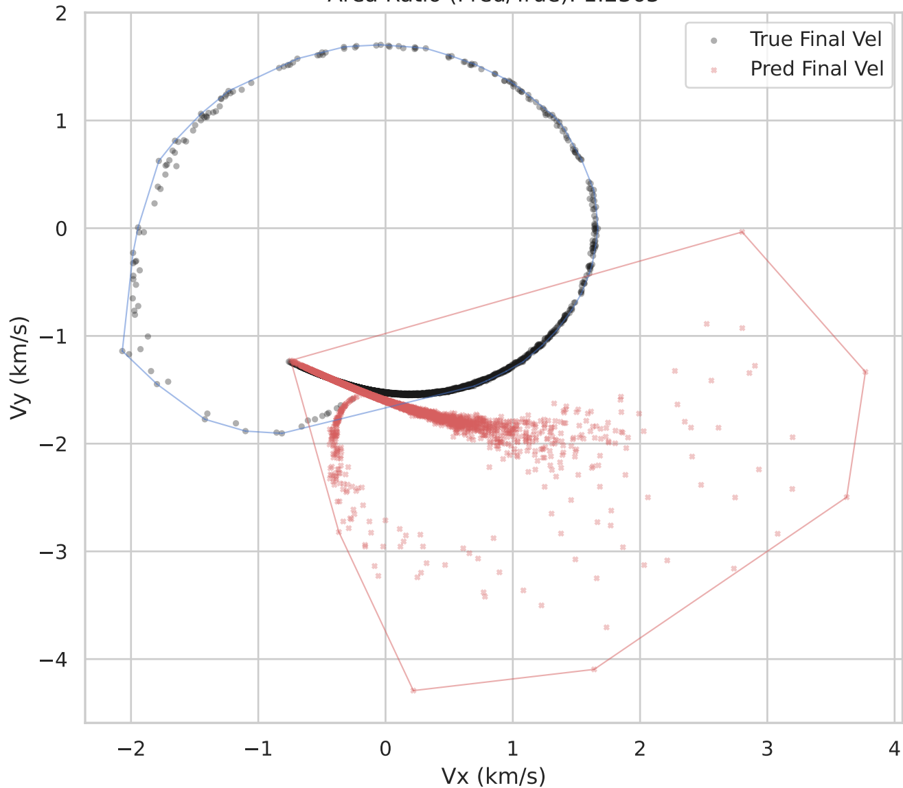
mamba Final State Velocities Convex Hull Area Ratio (Pred/True): 1.2363
