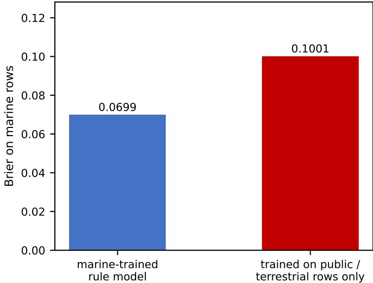
E Marine data advantage = 0.0302 (secondary success criterion)
