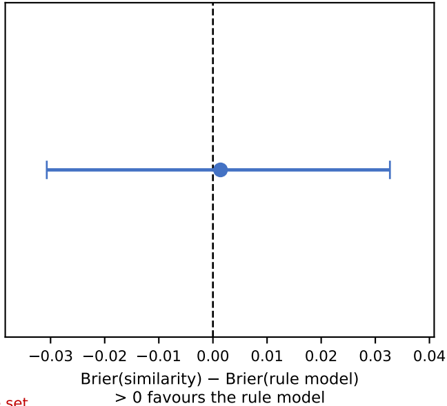
F Underpowered at n = 6 sealed compounds P(rule better) = 0.56, CI spans zero
