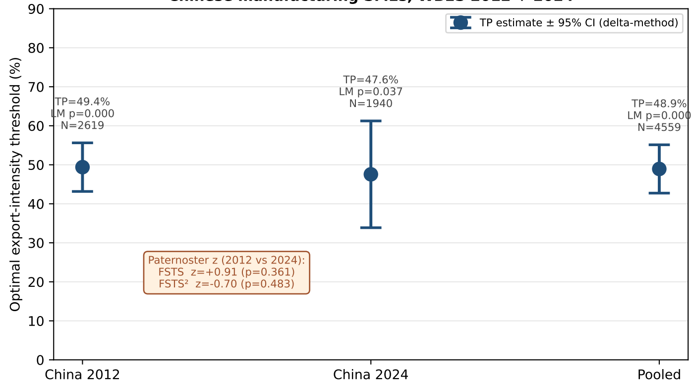
Figure 1. Stable export-intensity threshold across waves Chinese manufacturing SMEs, WBES 2012 + 2024
