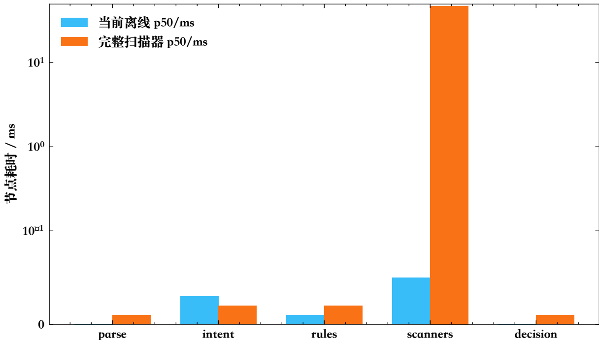
Pre-LLM pipeline 节点耗时分解
