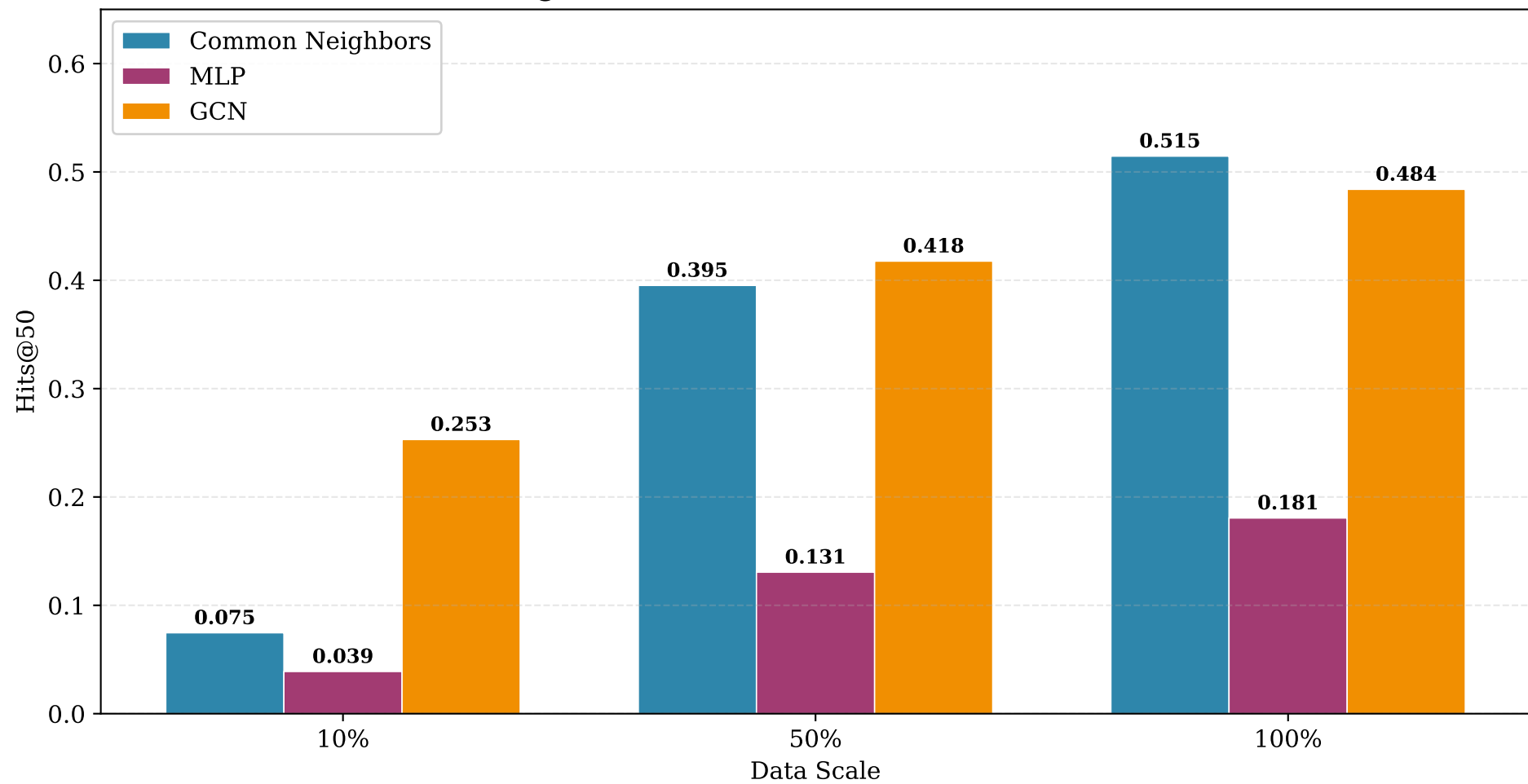
Hits@50 Performance: All Methods × All Scales
