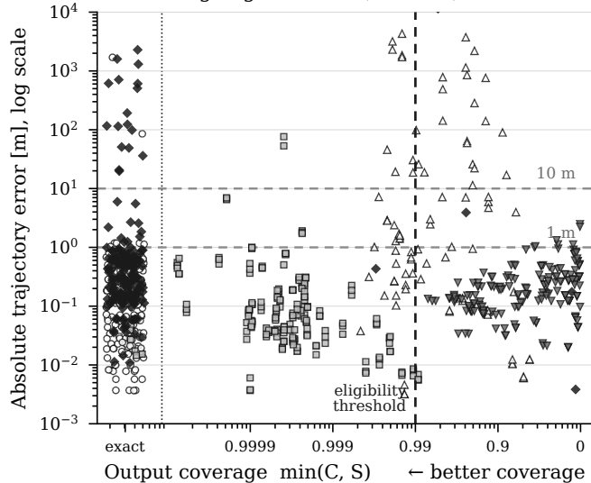
B Coverage against ATE (n = 861)
