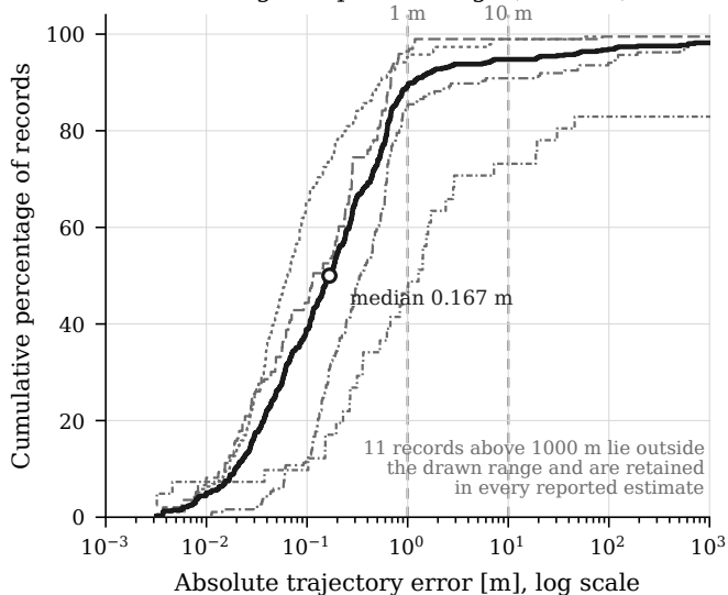
A ATE at high output coverage (n = 612)
