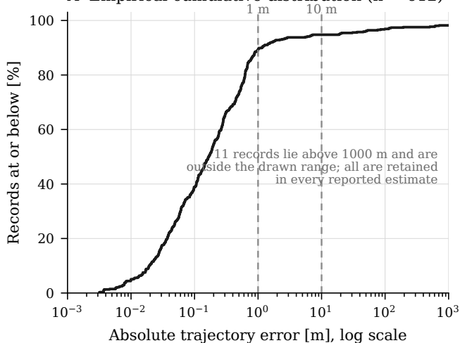
A Empirical cumulative distribution (n = 612)
