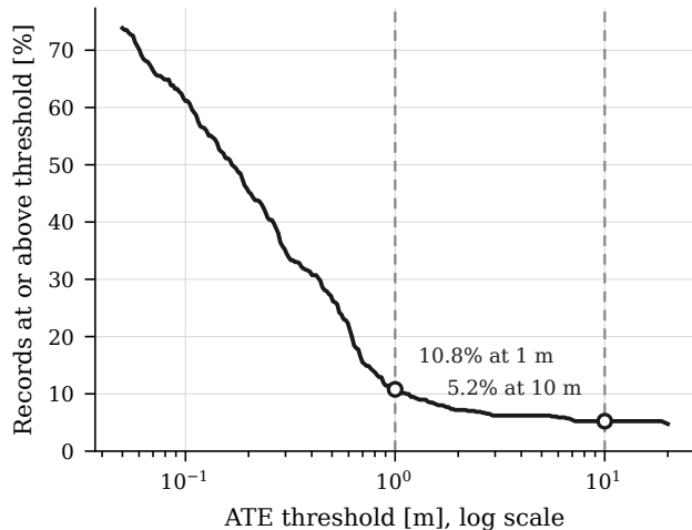
B Upper tail
