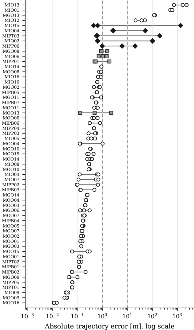
A ORB-SLAM3 (59 eligible triplets)
