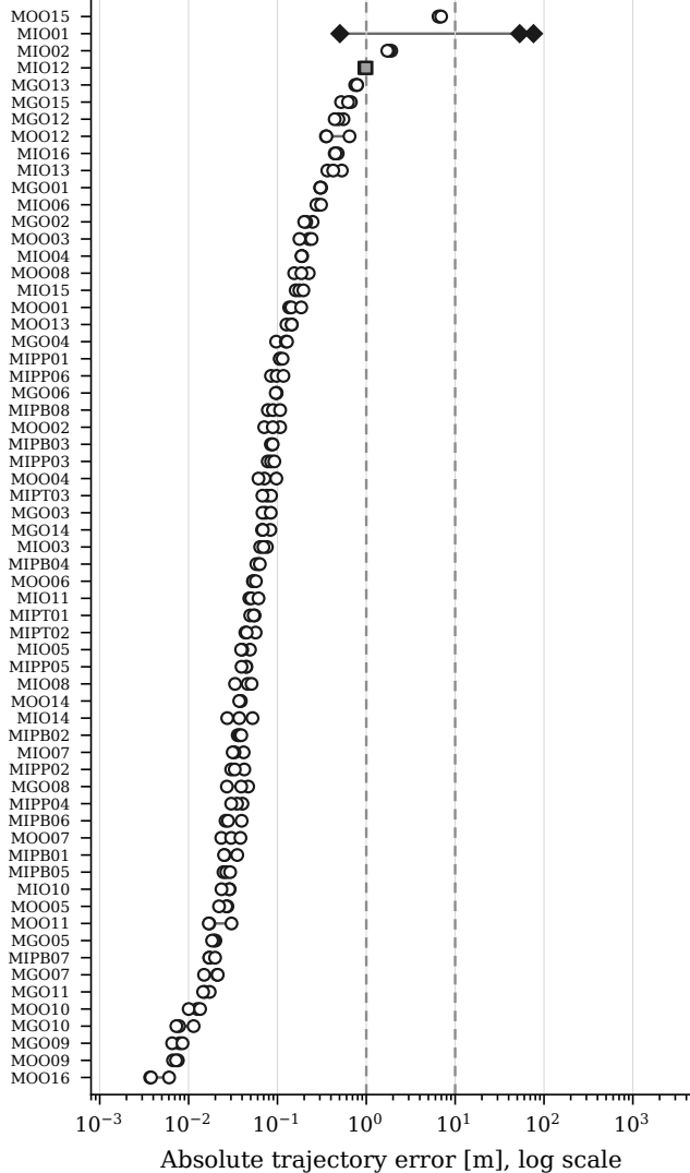
B OKVIS2 (63 eligible triplets)
