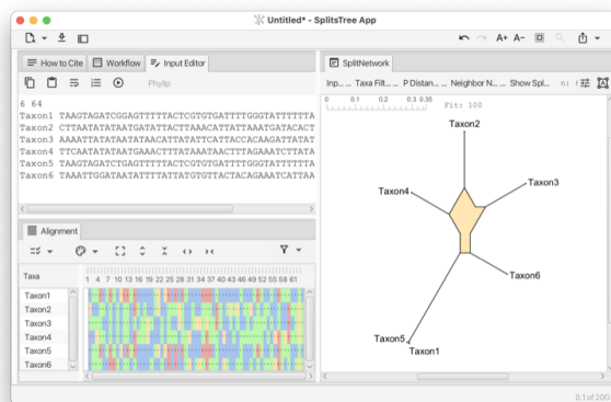
Figure 1.1: Neighbor net computed for toy characters data.
