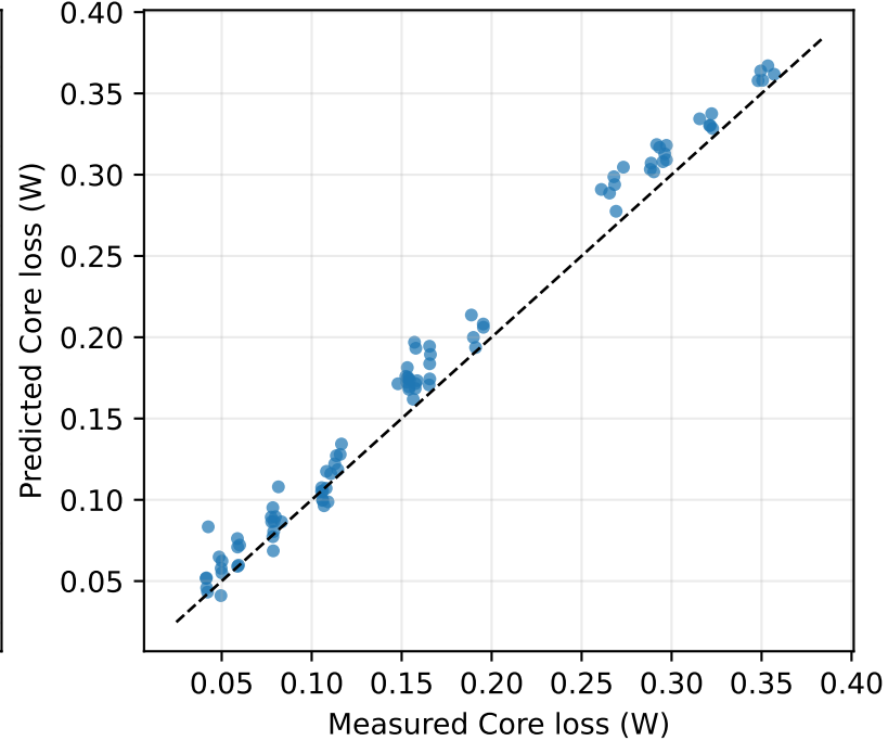
(b) Core loss
