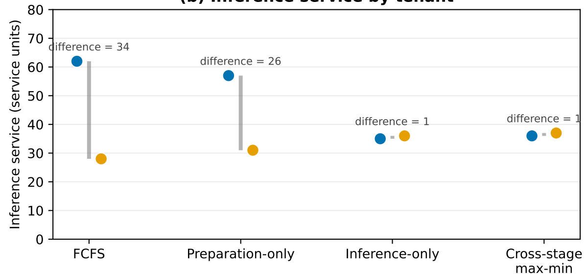
(b) Inference service by tenant
