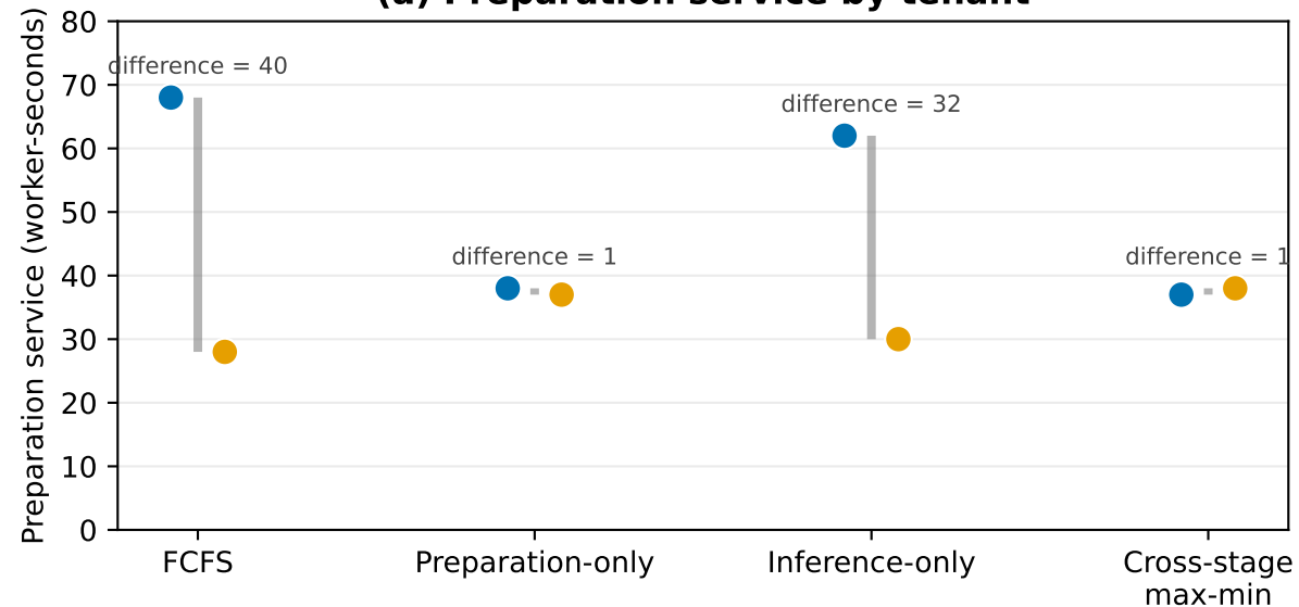
(a) Preparation service by tenant
