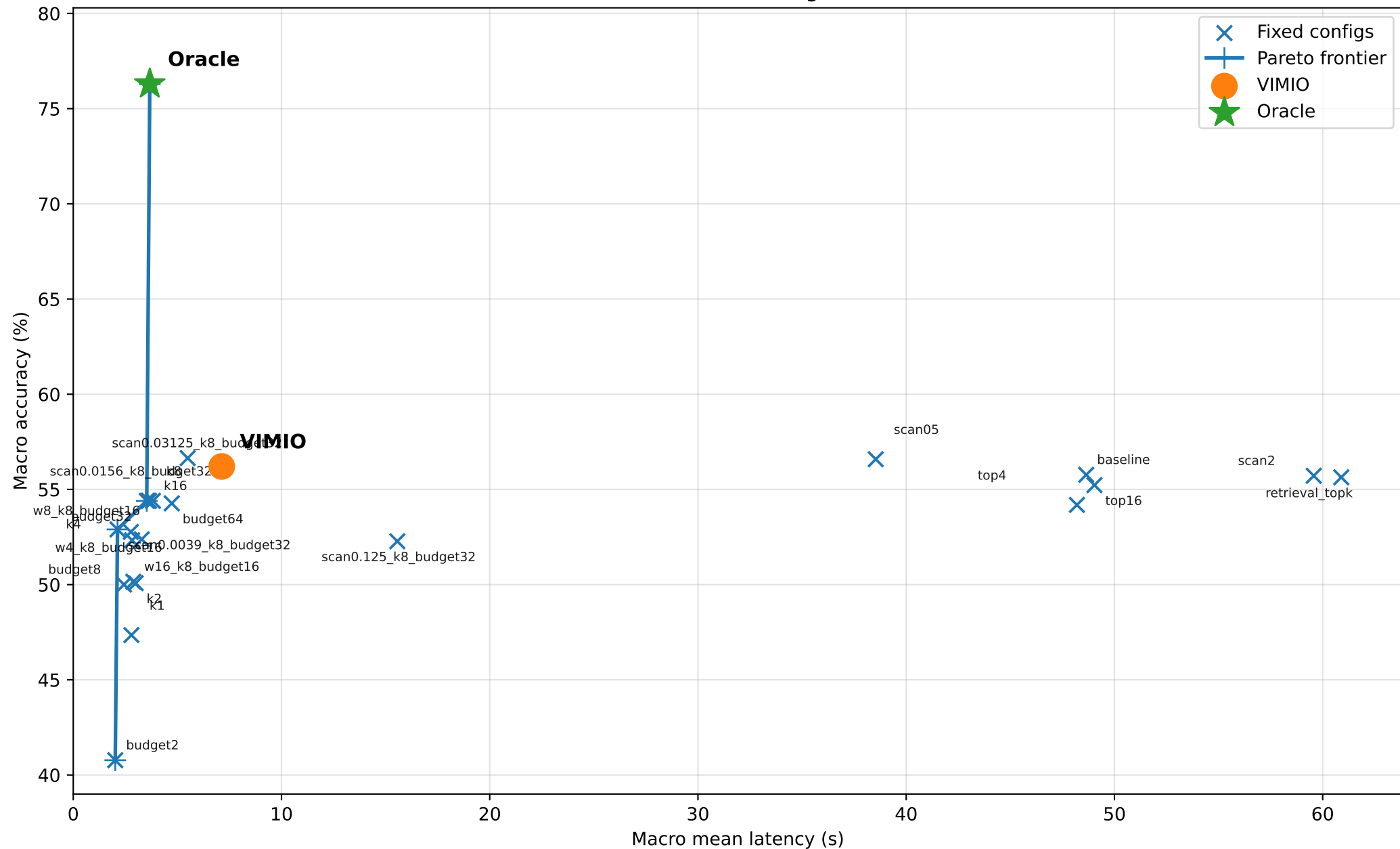
Consistent Evaluation: Fixed Configs, VIMIO, and Oracle
