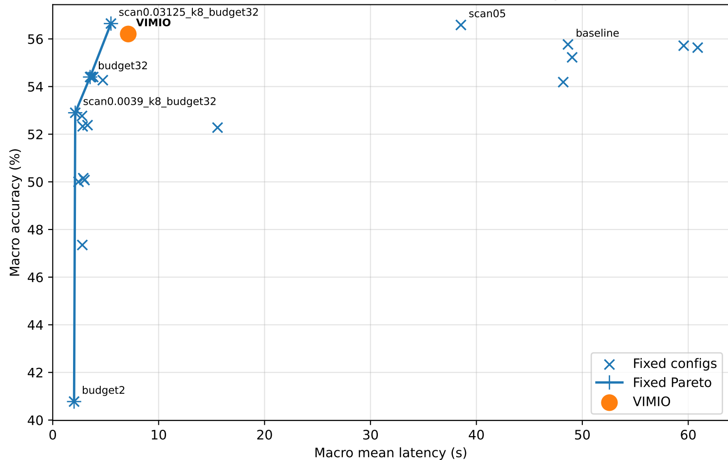
Consistent Evaluation: VIMIO vs Fixed Configs
