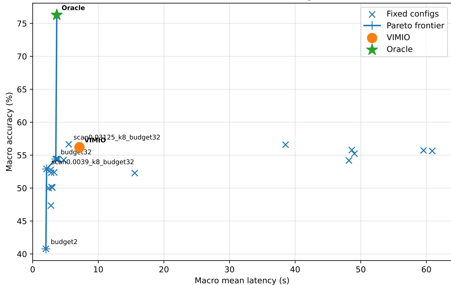
Consistent Evaluation: VIMIO, Fixed Configs, and Oracle
