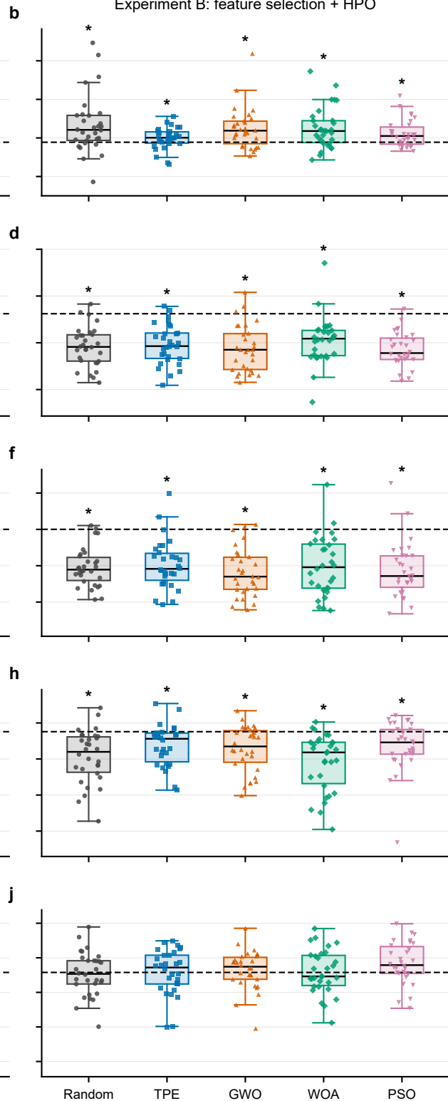
Experiment B: feature selection + HPO
