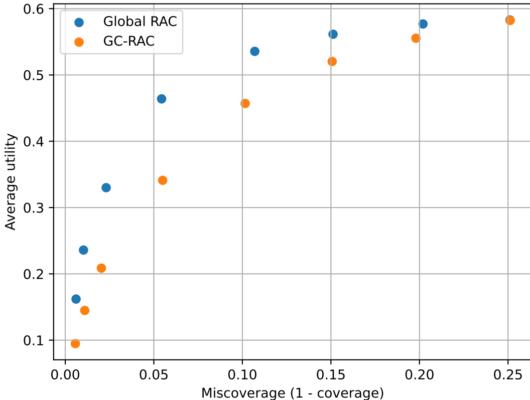
Pareto: Utility vs Miscoverage (each point is an \alpha )
