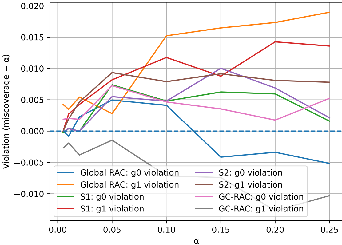
Per-Group Constraint Violations vs \alpha (All Methods)
