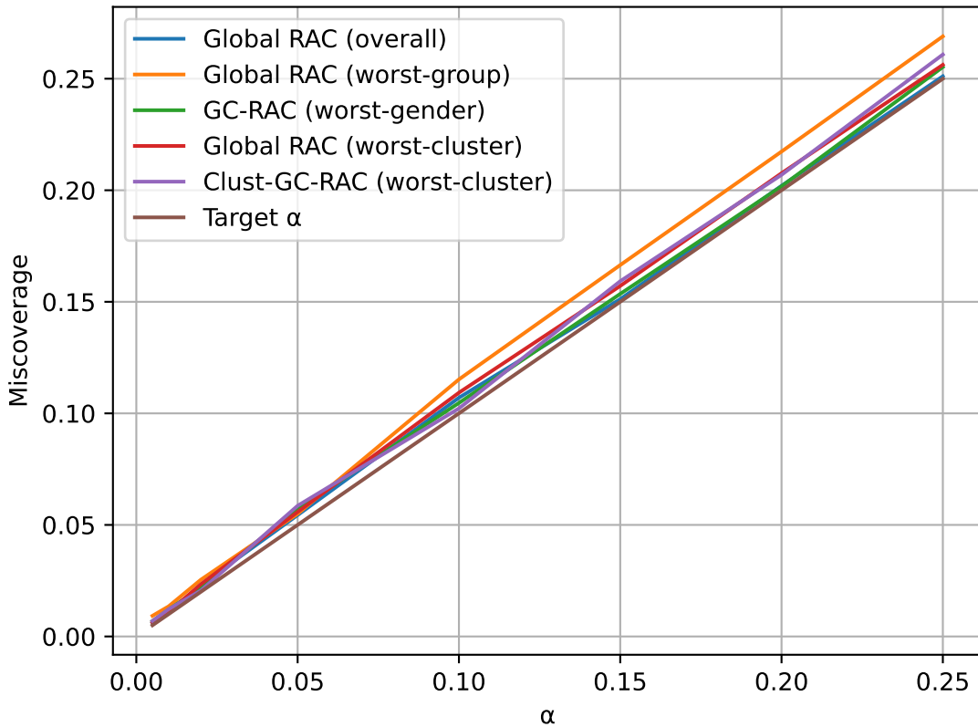
Worst-Group Miscoverage: Global RAC vs GC-RAC
